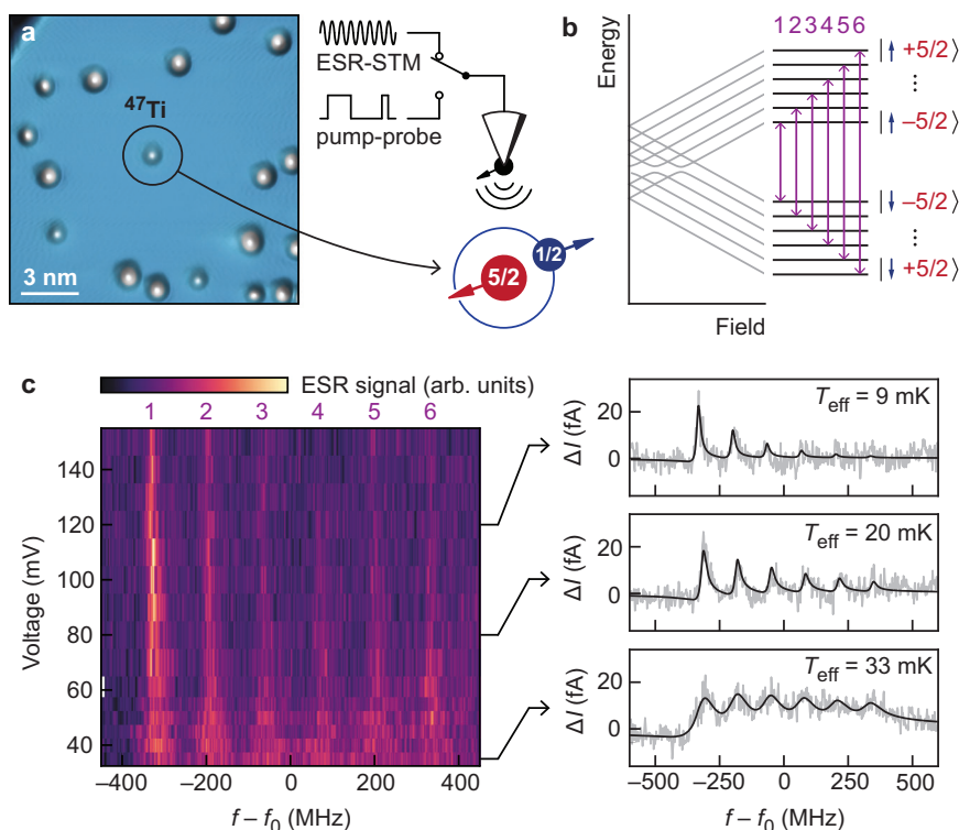
Fig. 1 | Single atom nuclear polarization. a STM topography of the single ^{47}\text{Ti} studied in this work. A schematic drawing shows the magnetic STM tip above the electron spin (blue) and nuclear spin (red) of the single atom. b Energy diagram of the spin states of a single ^{47}\text{Ti} . In the low field regime, avoided crossings appear between the different eigenstates. In the high field regime, the eigenstates resemble Zeeman product states. ESR transitions (purple arrows) can be driven between states with equal nuclear spin. c ESR-STM measurements at different
