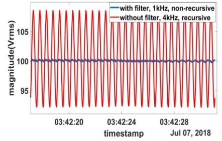
Figure 18. Magnitude estimation (Test B)
