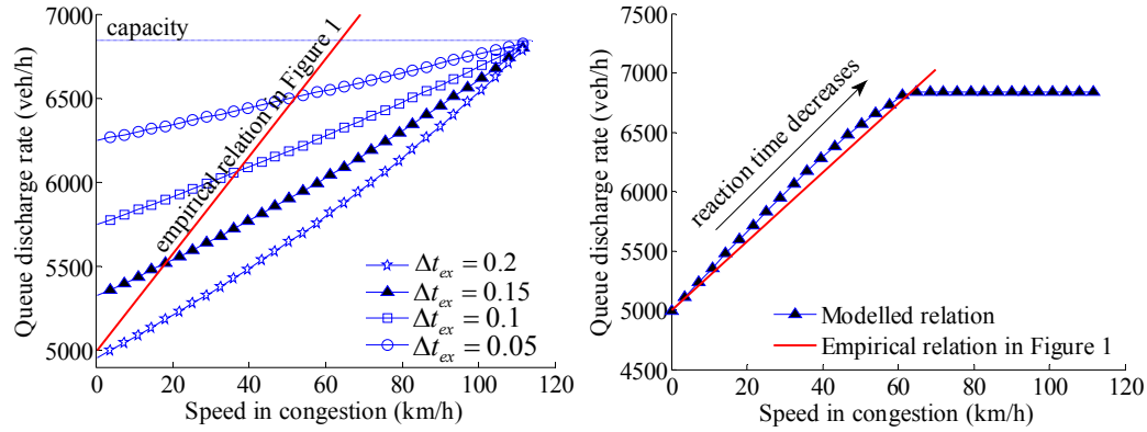
a) Sensitivity of the analytical model to the reaction time extension
