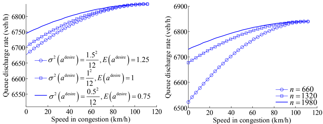
c) Comparisons of impacts on queue discharge rates between the mathematical expectation and the standard deviations of desired accelerations.
