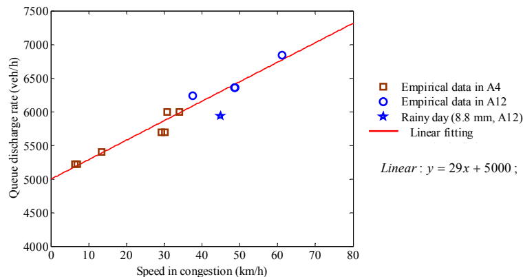
Figure 1 Relation between queue discharge rate and the speed in congestion [3].
