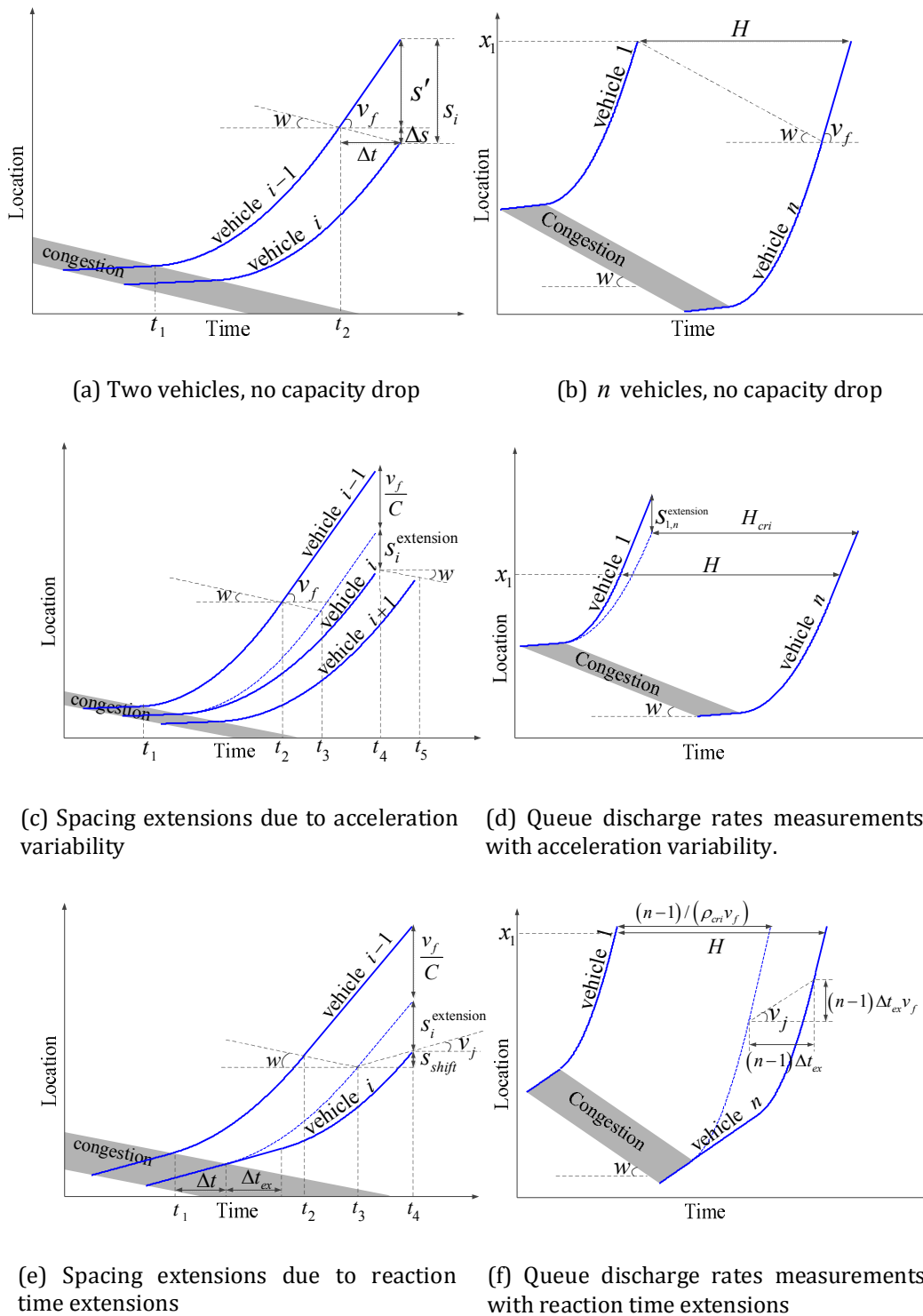
Figure 2 Measurements of queue discharge rates
