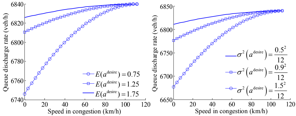
a) Sensitivity of the analytical model to the mathematic expectation of desired accelerations.
