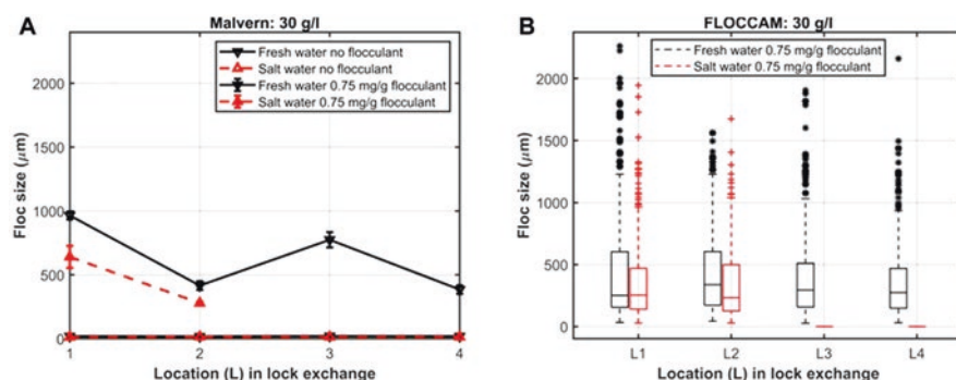
Fig. 7.16 Hydrodynamic size of ACCZ flocs at locations L1-L4 in the lock exchange. (a) Results obtained by SLS and (b) results obtained from FLOCCAM
