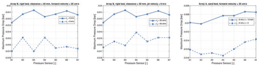
Fig. 7.5 Experimental results illustrating the effect of the jet velocity v_j (left), the forward velocity v_f (middle), and clearance c (right) on the maximum pressure drop under a Coandă-effect-based collector (Alhaddad et al., 2023). Pressure sensors B1-B7 and A1-A7 are spaced by a distance of 10 cm
