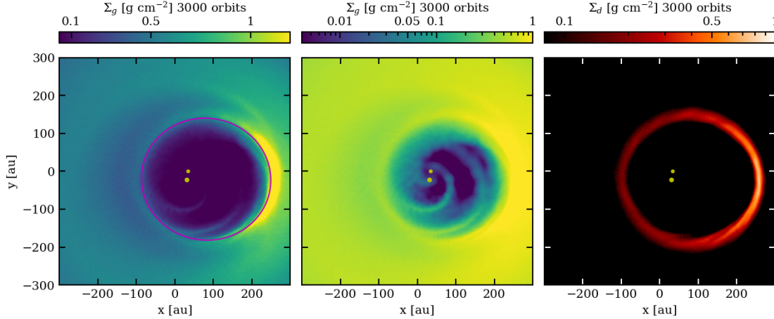
Fig. 7. Coplanar 1 simulation: same quantities as Fig. 5 for the longer timescale (3000 orbits), corresponding to \sim 4.9 \times 10^5 yr. The long-time evolution leads to the growth of eccentricity in the disc. Left and centre: gas surface density after 3000 orbits. Right: dust surface density. The dust is still trapped in the gas pressure maximum in an eccentric ring.
