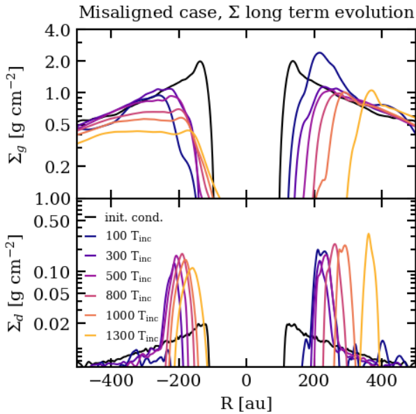
Fig. 8. Misaligned 1 case: radial cut along the major axis of the surface density profile of the gas (top, \Sigma_g ) and dust (bottom, \Sigma_d ) as a function of the distance of the star, R (au), for different time-steps. Initially, a low-eccentric ( e_{\text{cav}} \lesssim 0.03 ) cavity and dust ring form. Later on, the simulation shows a larger and more eccentric cavity and dust ring.
