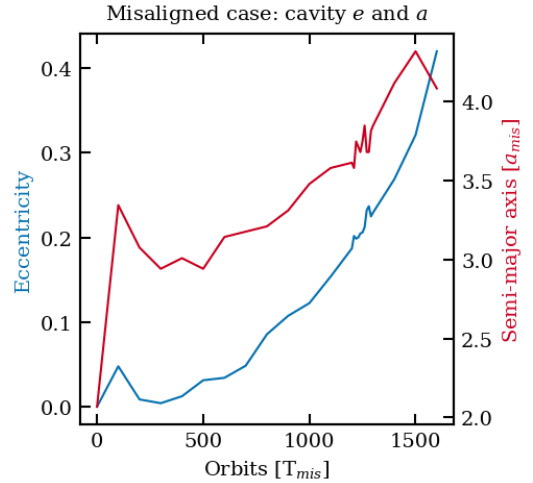
Fig. 9. Misaligned 1 simulation: evolution of the cavity semi-major axis, a , and the eccentricity, e_{\text{cav}} , as a function of the time, expressed in units of the period of the binary, T_{\text{mis}} . The values of e_{\text{cav}} and a increase after \sim 600 T_{\text{orb}} . It should be noted that the initial cavity size jump is due to the stabilisation of the initial conditions.
