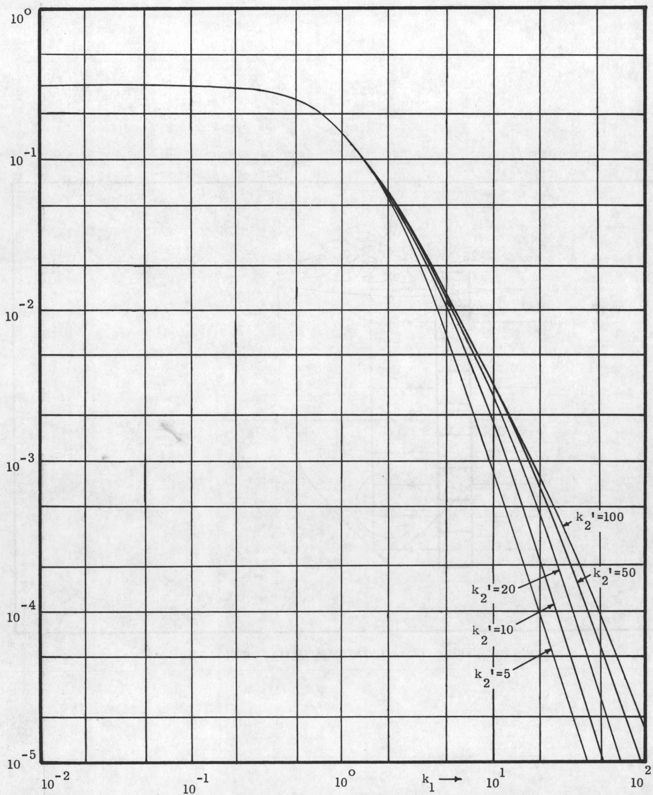
FIG. 9 SPECTRUM FUNCTION
