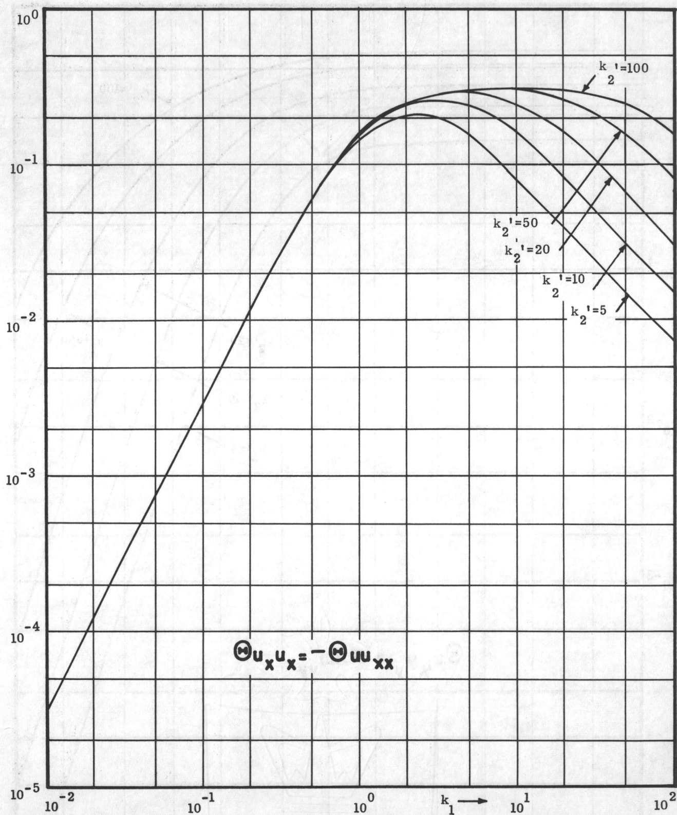
FIG. 16 SPECTRUM FUNCTION \Phi_{u_x u_x} L / \sigma^2
