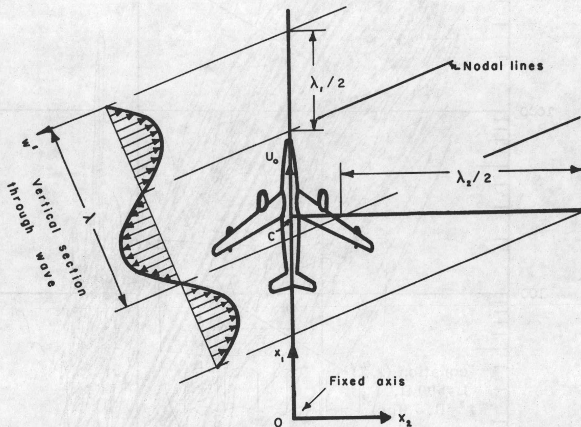
FIG. 7 THE VARIATION OF DOWNWASH IN THE x_1 x_2 PLANE FOR A SINGLE SPECTRAL COMPONENT
