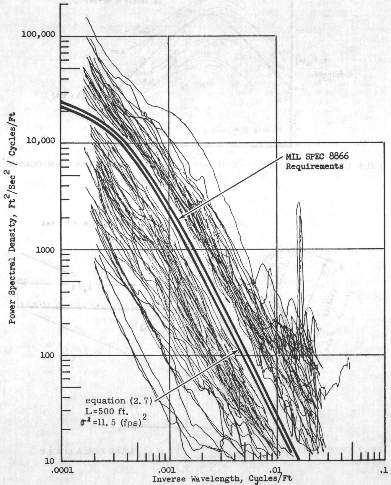
FIG. 5 COMPOSITE AND EXPECTED SPECTRUM OF FORWARD GUST VELOCITIES FROM TEST DATA AND MIL SPEC 8866 REQUIREMENTS (REPRODUCED FROM REF. 10, DOUGLAS AIRCRAFT CO.)
