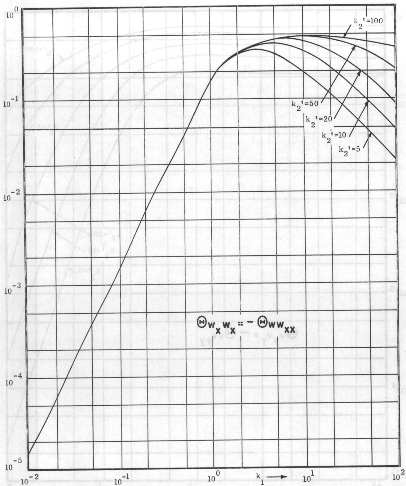
FIG. 21 SPECTRUM FUNCTION H_{w_x w_x} L / \sigma^2
