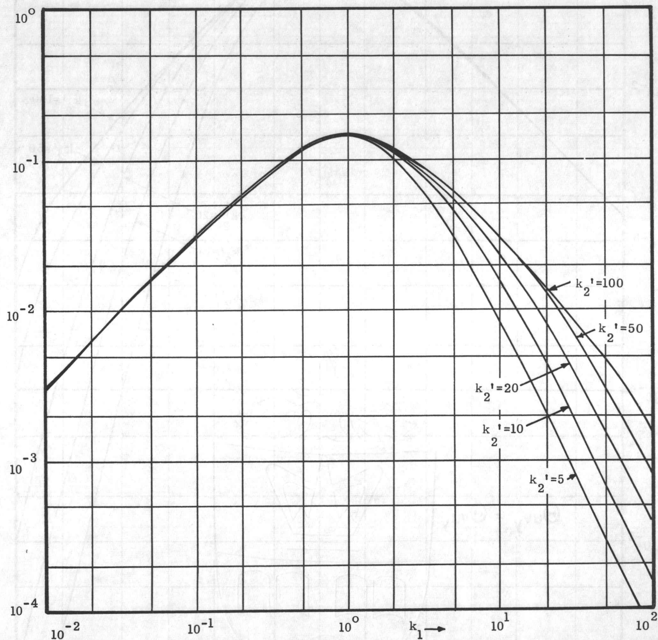
FIG.12 SPECTRUM FUNCTION \Theta_{uu_x}/i\sigma^2
