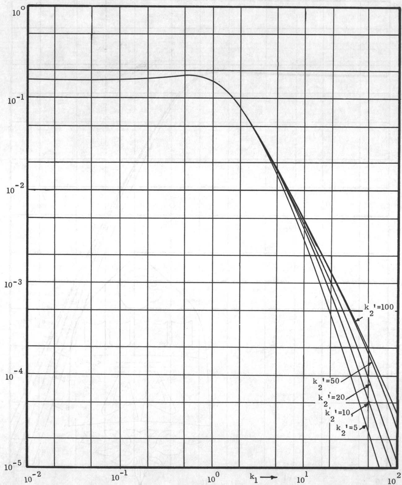
FIG.10 SPECTRUM FUNCTION \Phi_{vv}/\sigma^2 L
