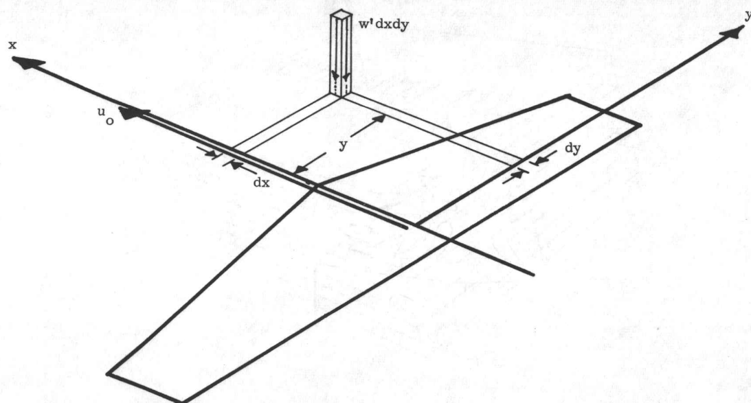
FIG.1 VERTICAL-GUST IMPULSE ( REPRODUCED FROM DIEDERICH, REF. 2)
