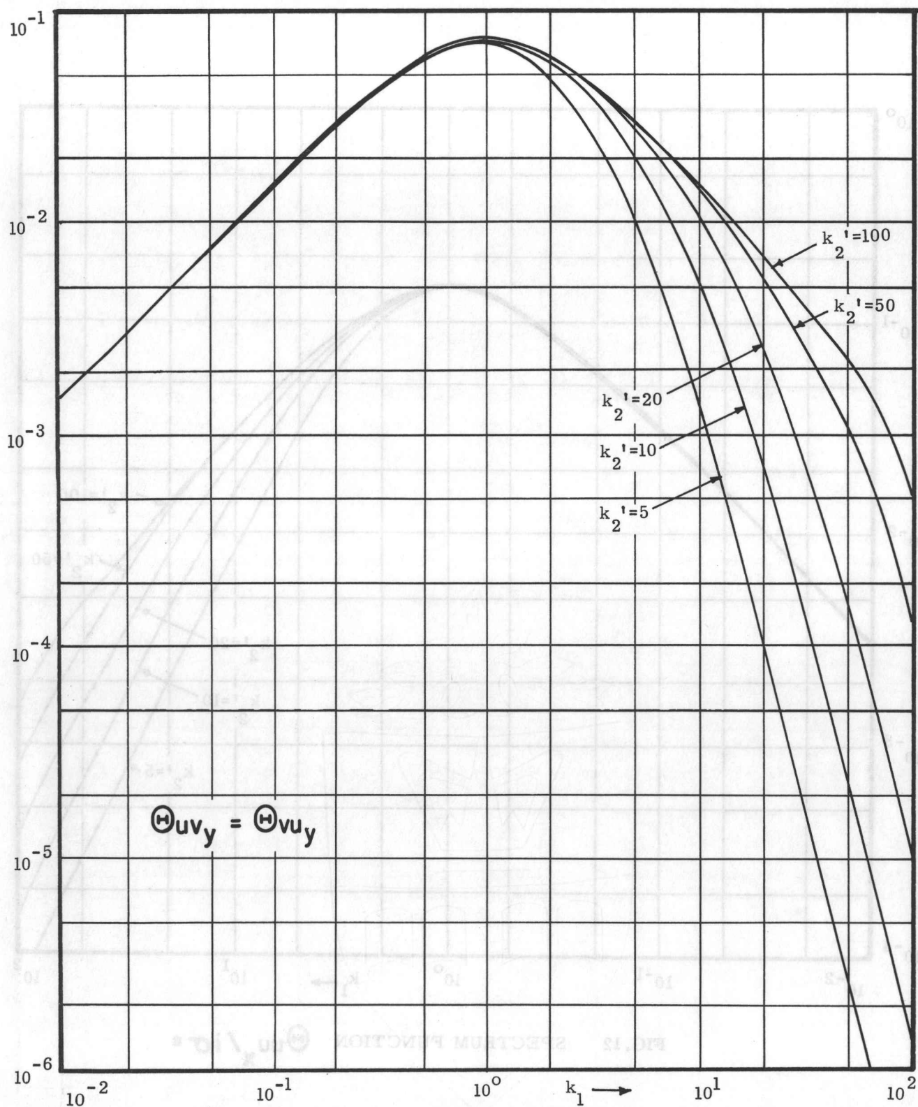
FIG. 13 SPECTRUM FUNCTION -\Phi_{uvy}/i\sigma^2
