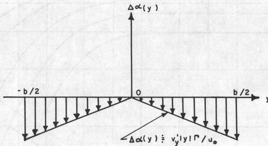
(a) \Delta\alpha distribution associated with v_y' .
