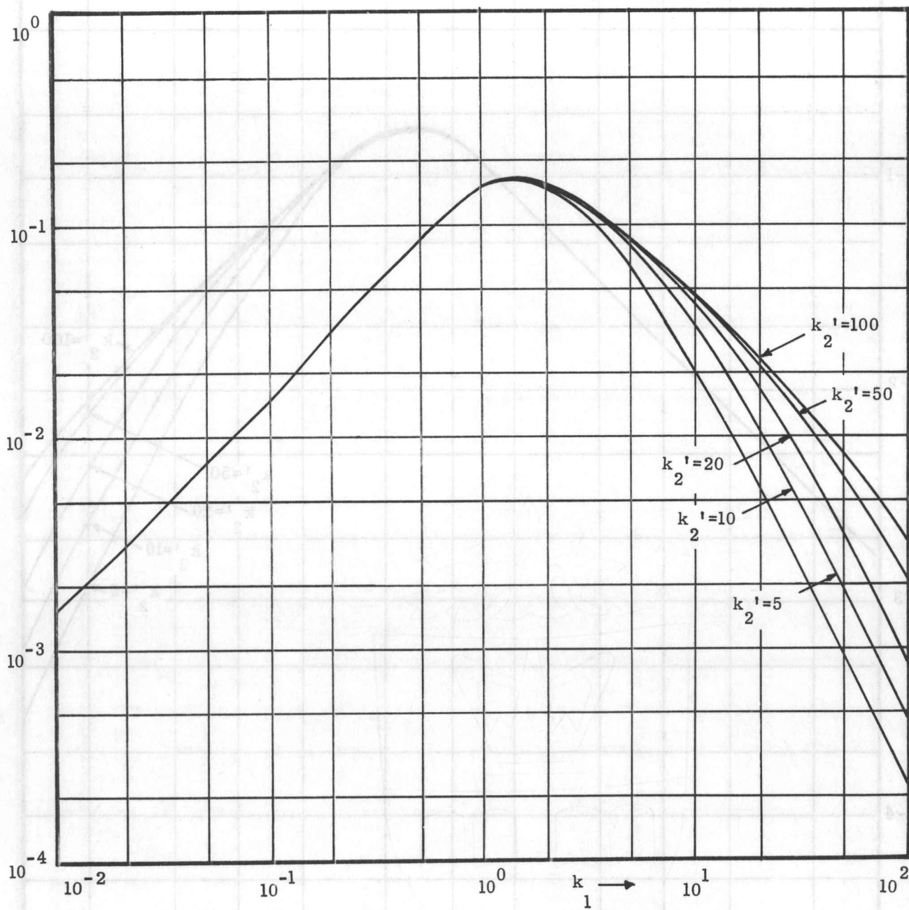
FIG.15 SPECTRUM FUNCTION H_{ww_x}/i\sigma^2
