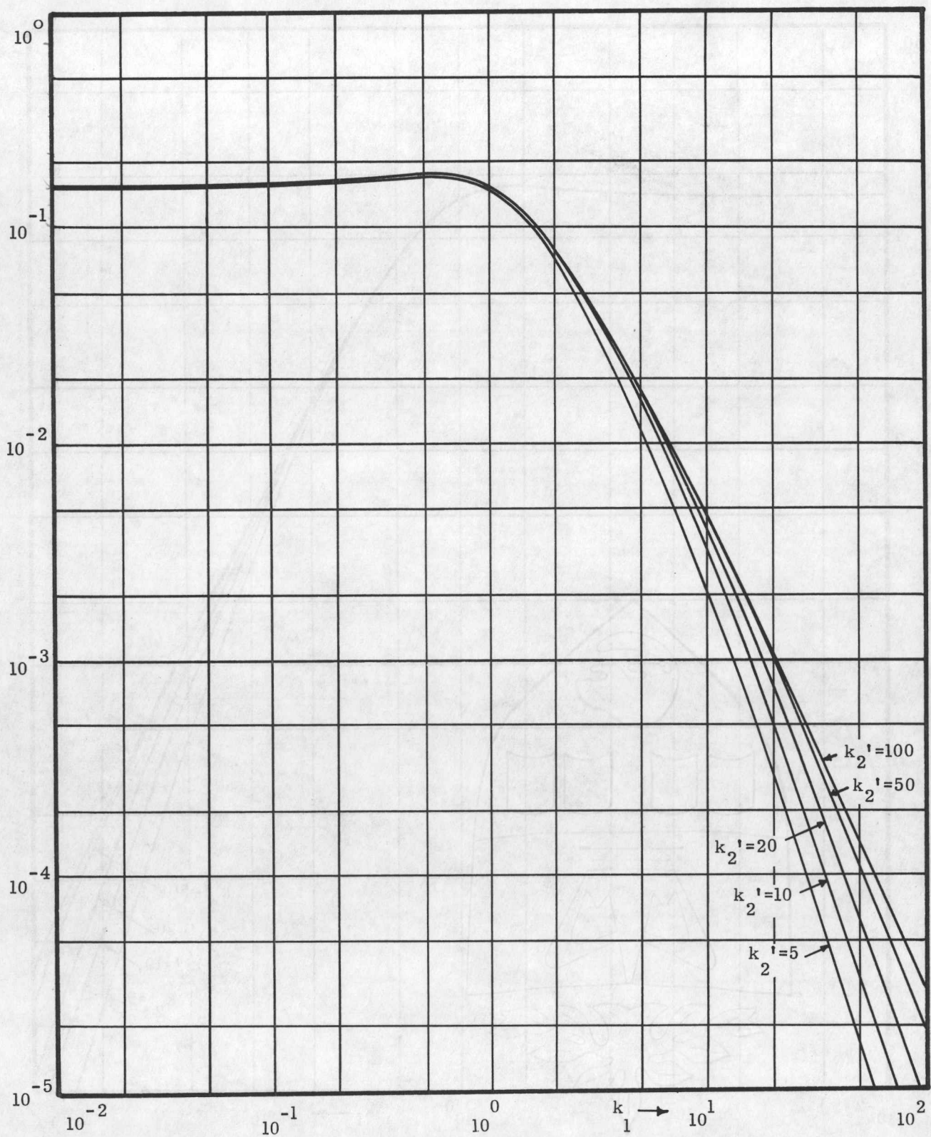
FIG. 11 SPECTRUM FUNCTION \Theta_{ww}/\sigma^2 L
