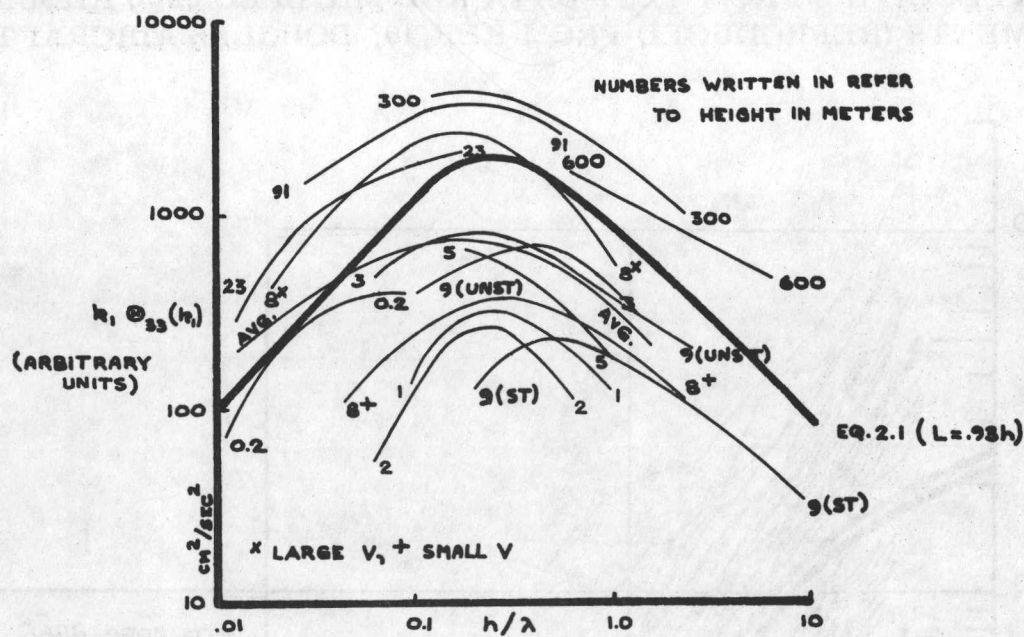
FIG. 6 LOW-LEVEL SPECTRA-COMPARISON OF DATA OF PANOFSKY & McCORMICK, REF. 11, WITH EQUATION 2.1
