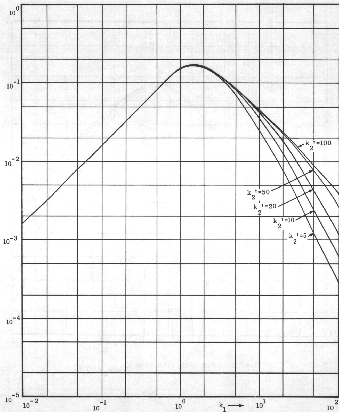
FIG. 14 SPECTRUM FUNCTION
