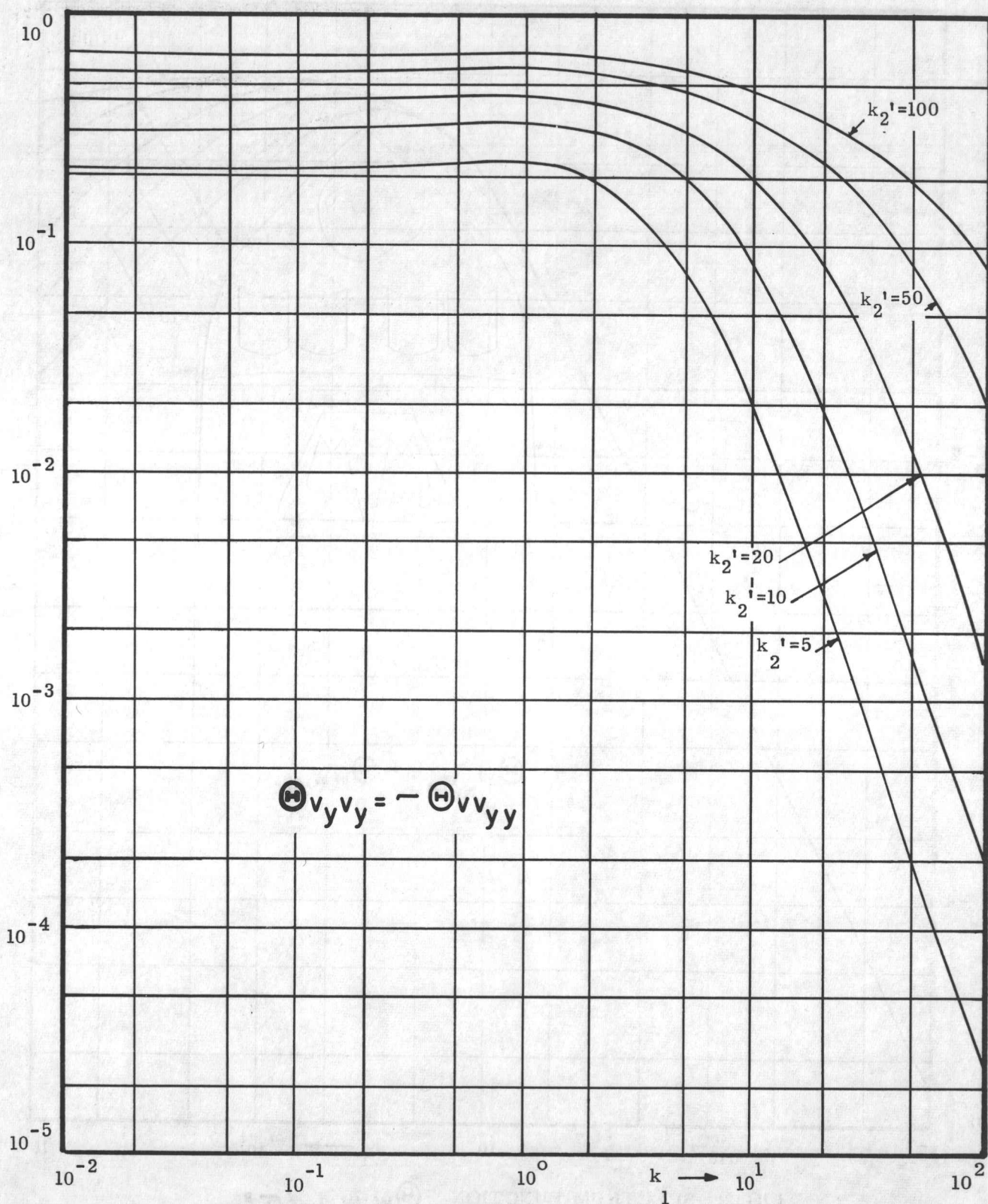
FIG. 20 SPECTRUM FUNCTION
