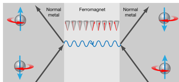
FIG. 1: Generation of a magnon (directional wavy line and snapshot of the magnetization) by the spin-transfer torque, which is associated with an electron spin flip indicated by spheres, at the left interface between normal metal and ferromagnet, and the reciprocal magnon detection by spin pumping at the right interface. (Credit: Alan Stonebraker)
