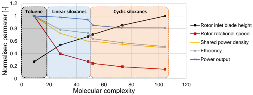
Figure 3.11: Normalised output parameters with respect to the maximum values versus molecular complexity, \sigma = T_{cr}/R(\partial S/\partial T)_{su,T_r=0.7} , of the six working fluids optimised in this paper.
