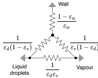
Figure F1: Radiative heat transfer network model.
