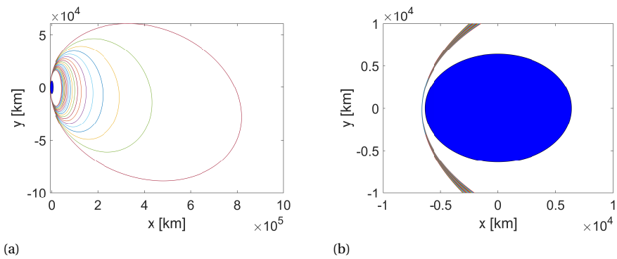
Figure G.4: (a) Example of spacecraft trajectory starting from general Ariane 5 GTO. The blue circle represents Earth. (b) Zoomed in schematic showing perigee.
