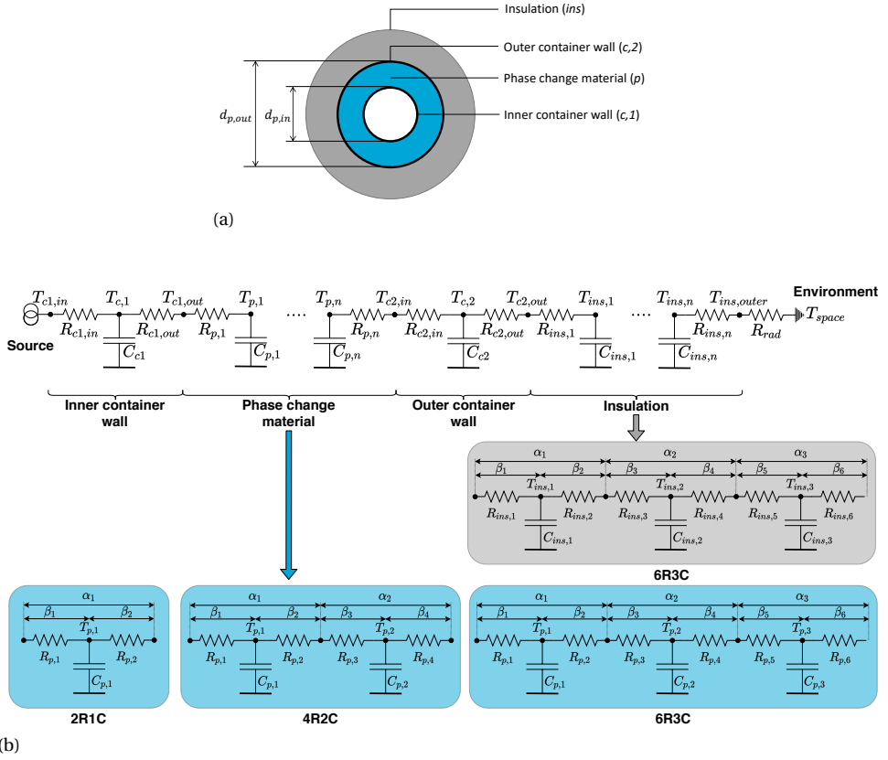
Figure 5.2: (a) Cross-sectional view of receiver. (b) Thermal nodal network of the receiver.
