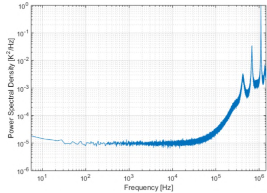
Fig. 5. PSD of 2^{19} bitstream samples, averaged over 100 cycles.
