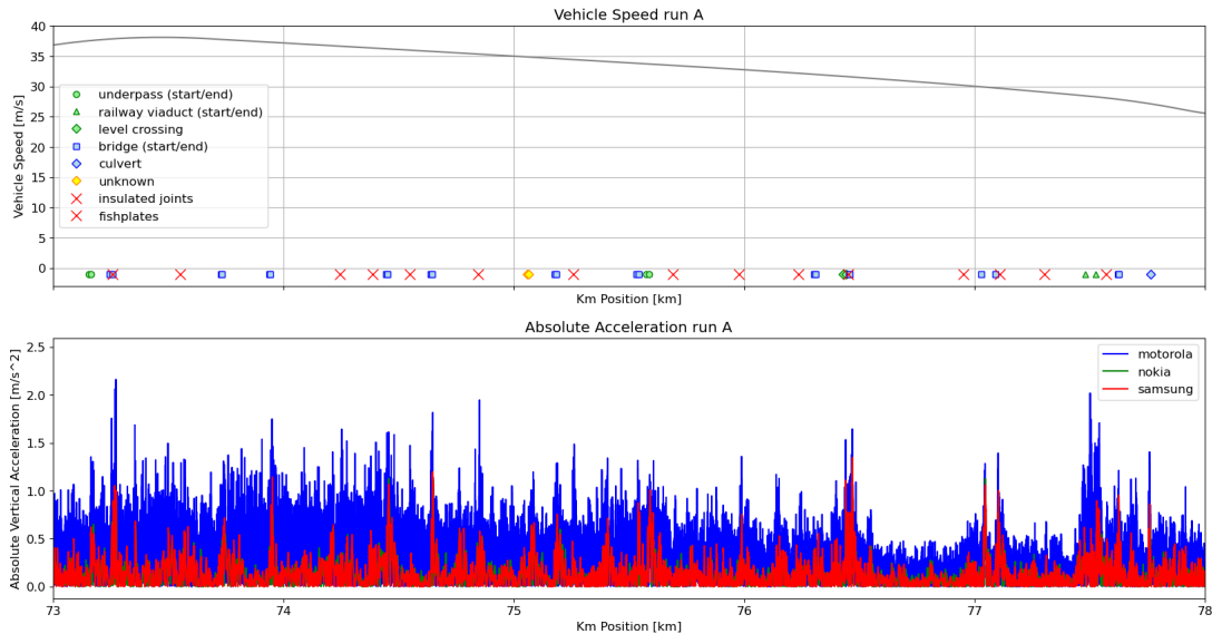
Figure 4.17: Speed profile run A, with the absolute vertical accelerations (minus the mean acceleration for the run) per phone.
