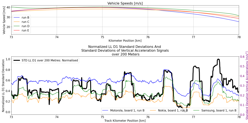
Figure 5.1: Standard deviations of the track geometry parameters versus the vertical accelerations of the mobile phones for the smartphones on board 1. The top plot displays the vehicle speed of the various runs.
