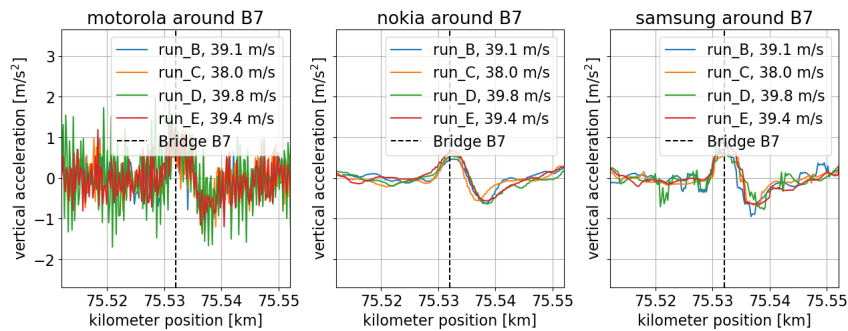
Figure 4.14: Vertical accelerations of smartphones of board 1 on different measurement runs around bridge B7.
