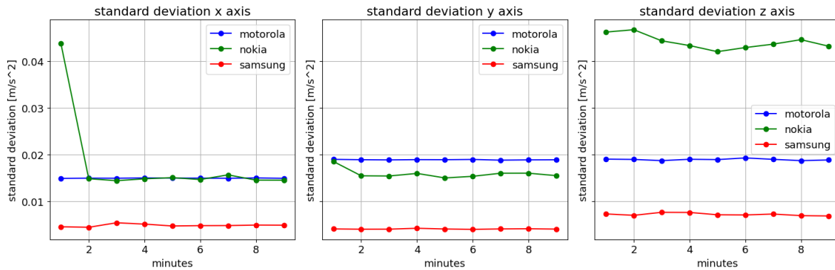
Figure 3.5: Standard deviation per minute, per axis, per smartphone
