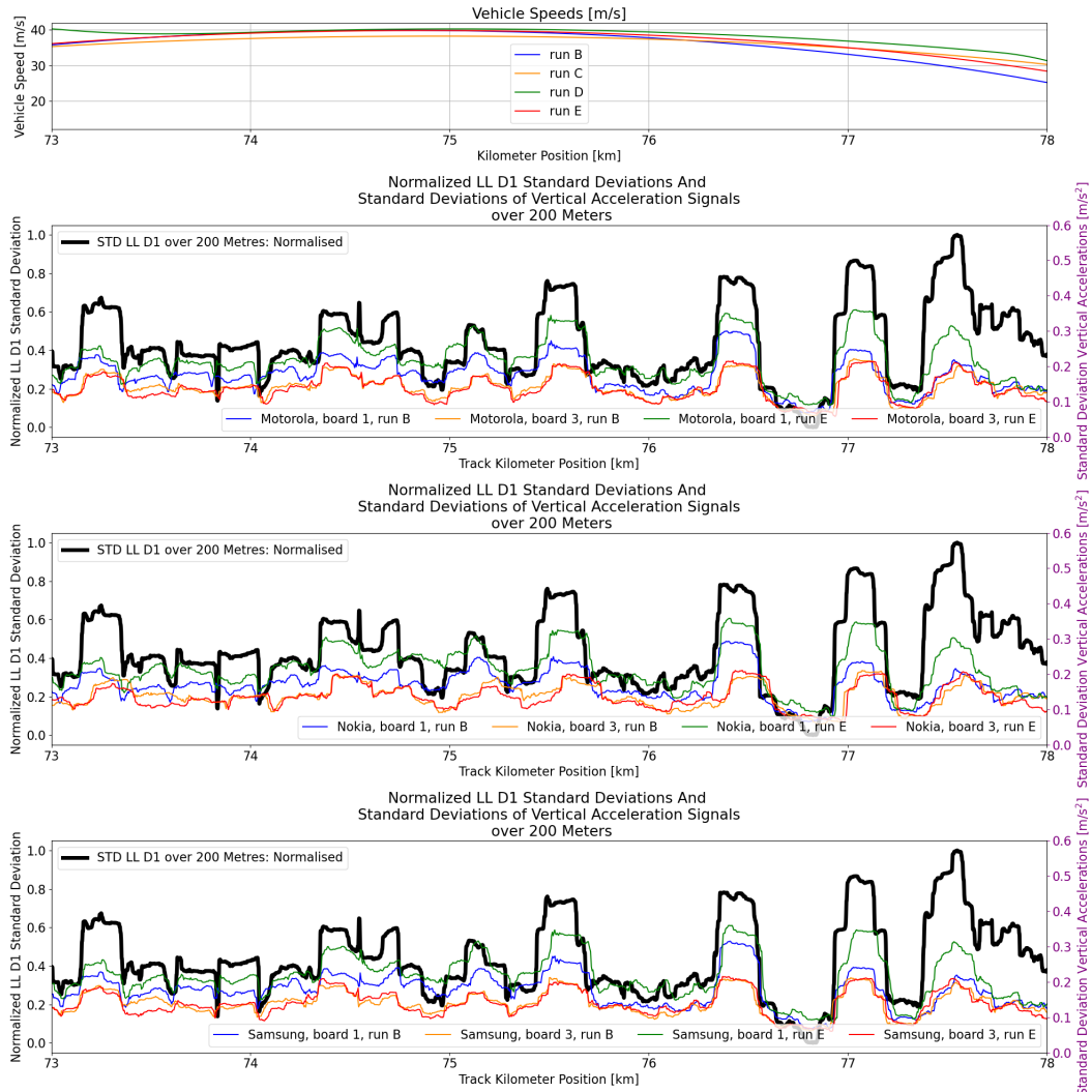
Figure 5.3: Standard deviations of the track geometry parameters versus the vertical accelerations of the mobile phones for the smartphones on board 1 and 3. The top plot displays the vehicle speed of the various runs. Depicted are the results for runs B and E.
