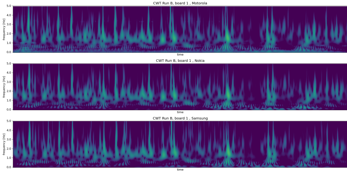
Figure 4.8: CWT of the vertical accelerations of the smartphones on board 1 for run B.
