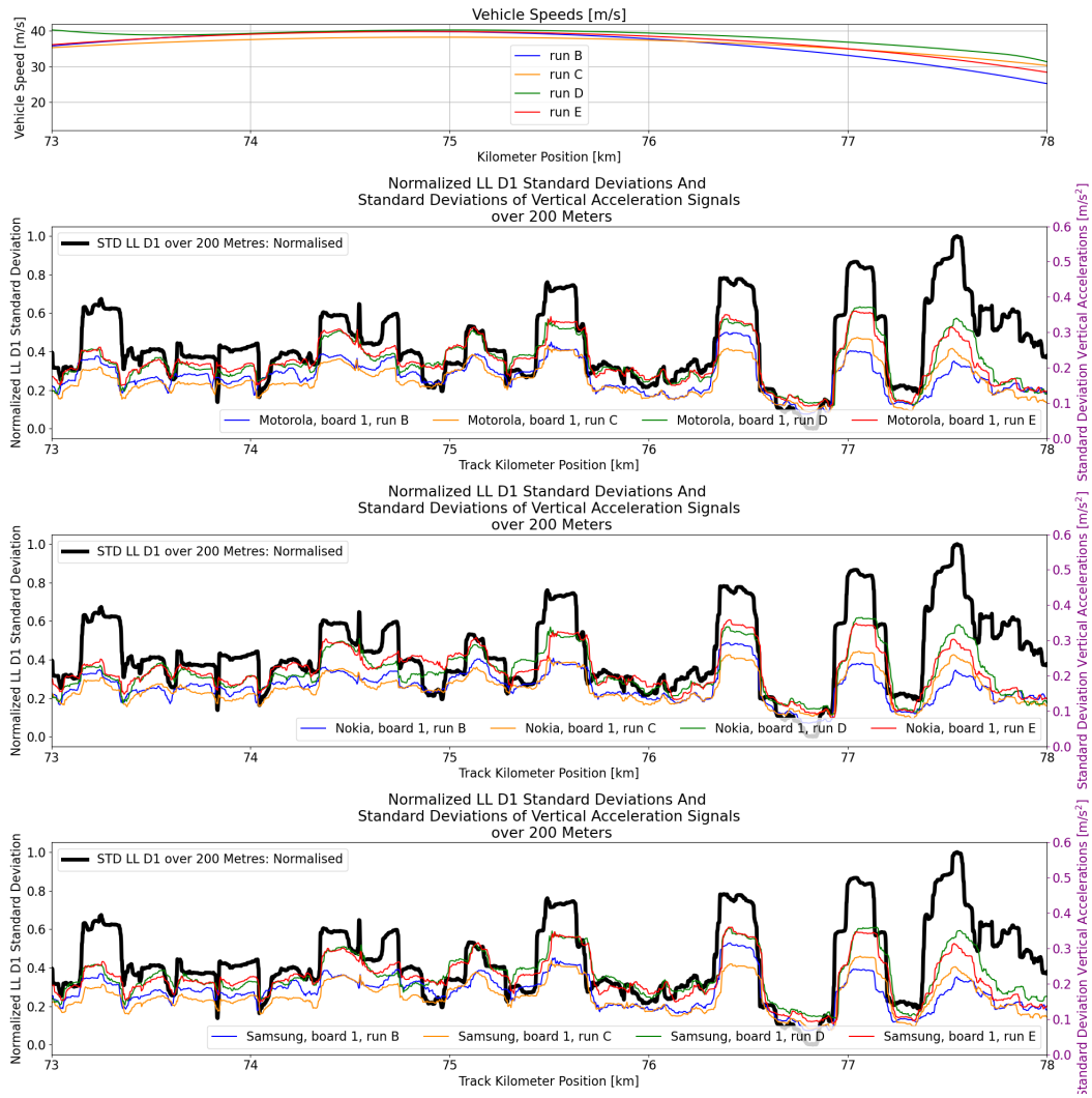
Figure 5.2: Standard deviations of the track geometry parameters versus the vertical accelerations of the mobile phones for the smartphones on board 1. The top plot displays the vehicle speed of the various runs. The vertical acceleration filters have been low-pass filtered for 5 Hz.
