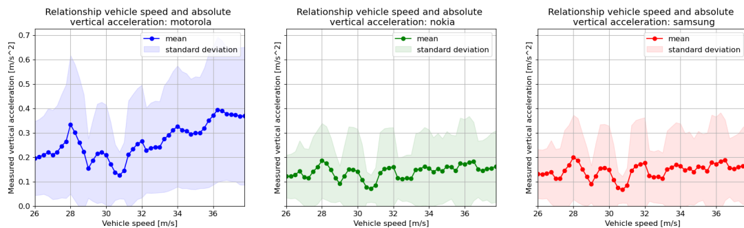
Figure 4.18: Vehicle speed versus absolute vertical acceleration per smartphone. The means are calculated by dividing the datapoints up into bins of size 0.25 m/s
