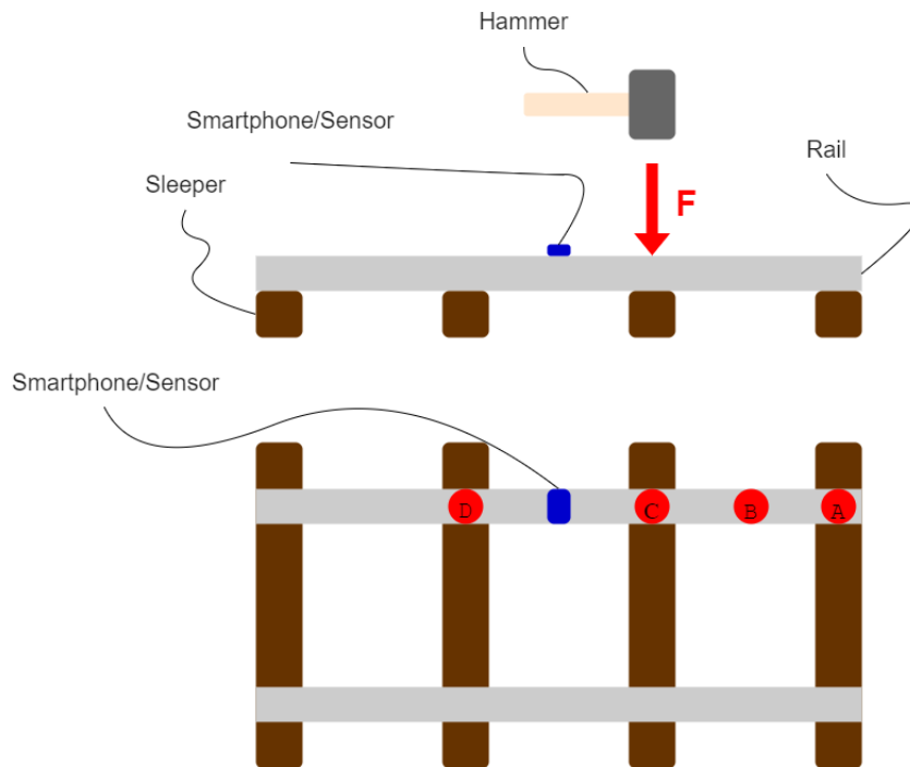
Figure 3.10: Schematic of the impact location. The impact location used in this thesis was location C.
