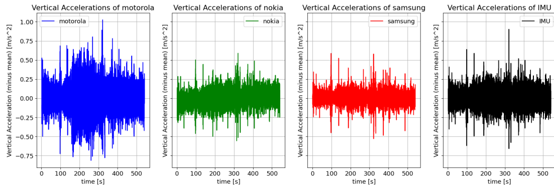
Figure 3.15: Vertical accelerations per measurement device. A clear trend is again visible in the Nokia.
