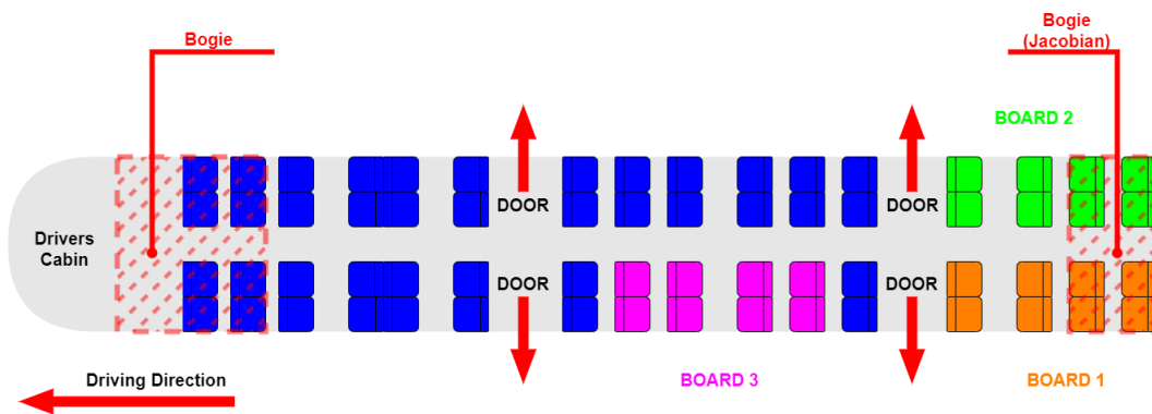
Figure 4.3: Location within car body of the measurement boards on a schematic overview of the car body. In Measurement run A, only Board 1 was instrumented. The bogies and target seats are indicated.
