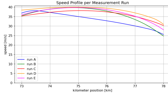
Figure 4.11: Speed curves of the different runs.
