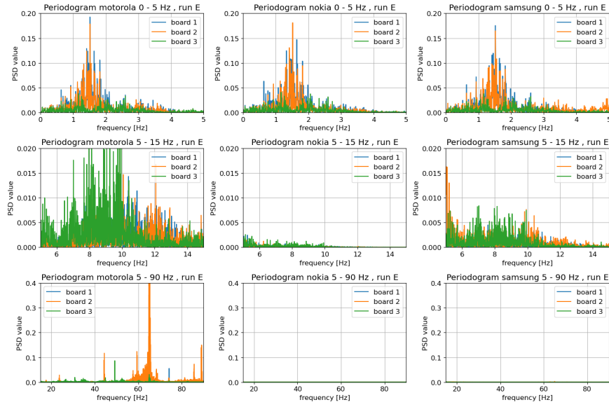
Figure 4.22: Periodograms for the different smartphones, for different boards in run E.
