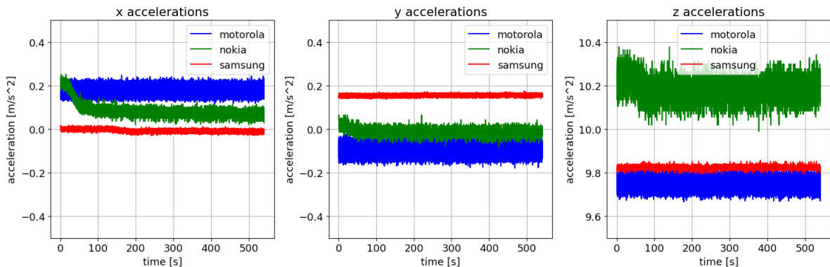
Figure 3.3: Raw accelerations of all three axes for each smartphone
