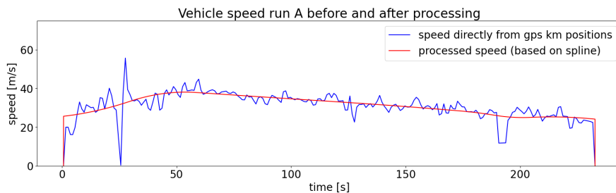
Figure 4.5: Speed profile based on GPS recordings of the iPhone for measurement run A. In blue: the speed profile based on track kilometer positions of the iPhone. In red: the speed profile after the track kilometer positions after a univariate spline was applied.
