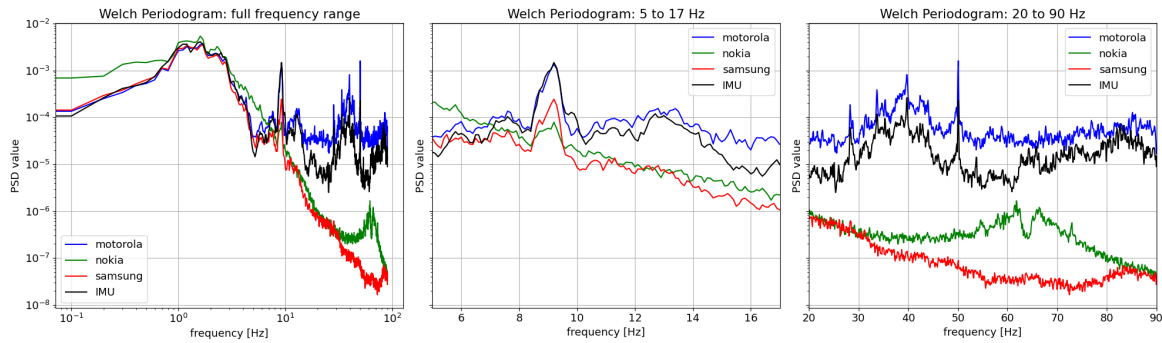
Figure 3.14: Welch-Periodogram of all the measurement devices for different frequency ranges
