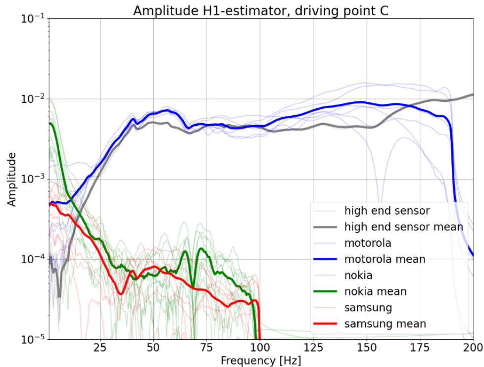
Figure 3.11: The amplitudes of the H1-estimators for the different measurement devices. The thin, semi-transparent lines represent the individual FRF-curves, whilst the thicker lines represent their means. The high-end sensors are represented by a grey line, the Motorola by blue, the Nokia in green and the Samsung in red.
