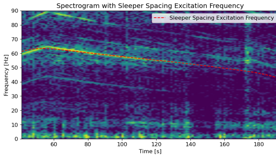
Figure 4.10: Spectrogram of Motorola in run A, with sleeper spacing frequencies based on the speed and sleeper spacing indicated with lines.
