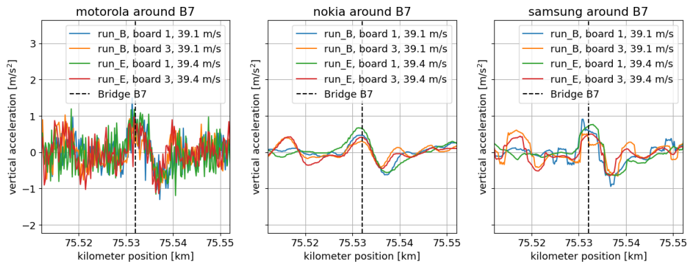
Figure 4.21: Vertical accelerations around bridge B7. Signals are aligned manually around the peak visible around B7.
