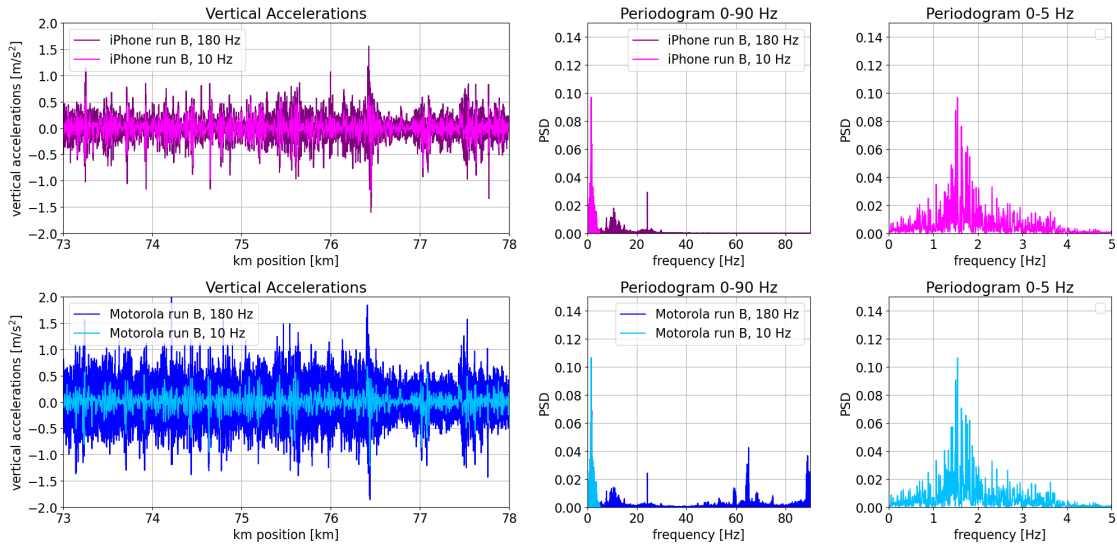
Figure 5.4: Vertical signals of the iPhone and the Motorola for run B. The maximum sampling frequency of the iPhone was 50 Hz, hence the lack of frequency content in the periodograms past 50 Hz for this device.
