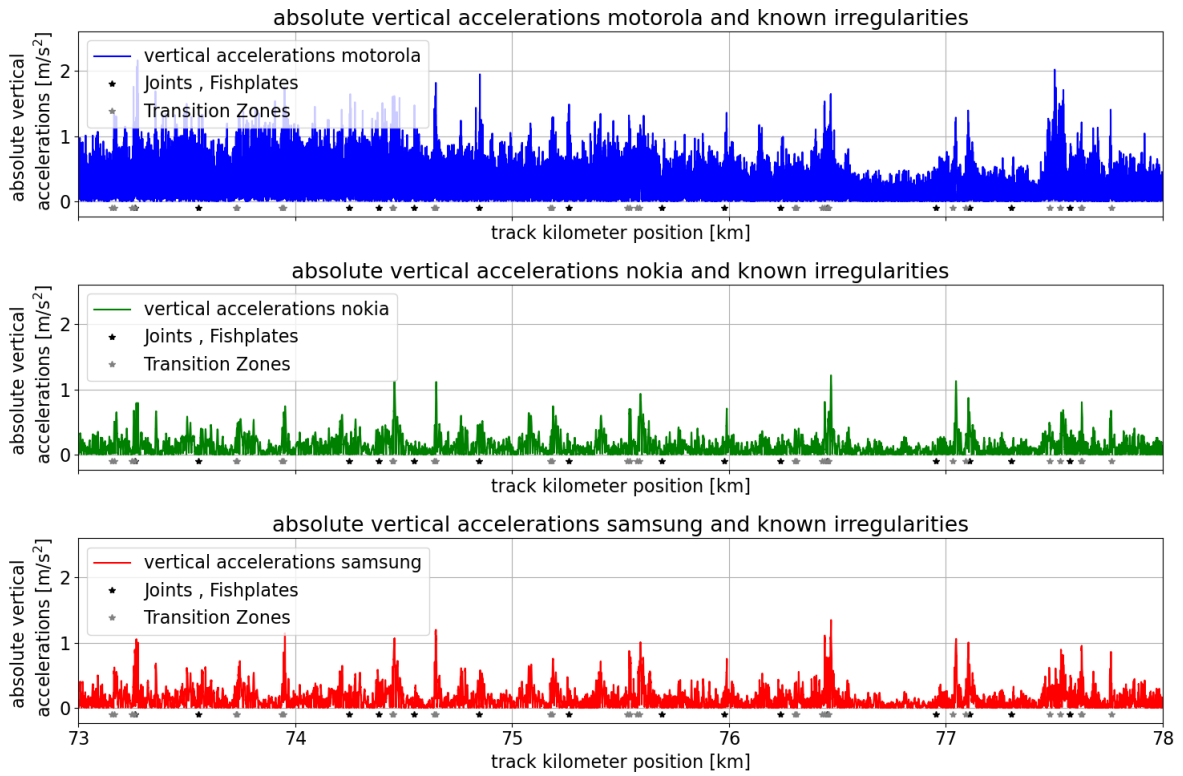
Figure 4.9: Absolute vertical accelerations versus the kilometer position for each device in the test set. Data is taken from measurement run A. All infrastructure elements (joints, transition zones) are plotted.
