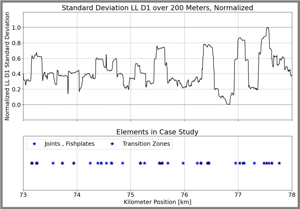
Figure 1.4: Track Quality Index. The standard deviation over 200 meters of the LL D1 is presented normalised over the track segment, with a value of 0 meaning the best TQI score on this segment and a 1 meaning the worst TQI score on this segment. The locations of transition zones and joints are provided for additional context.
