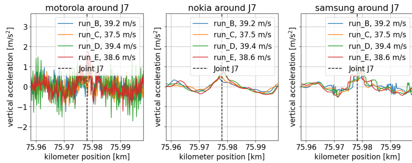
Figure 4.13: Vertical accelerations of smartphones of board 1 on different measurement runs insulated joint J7.
