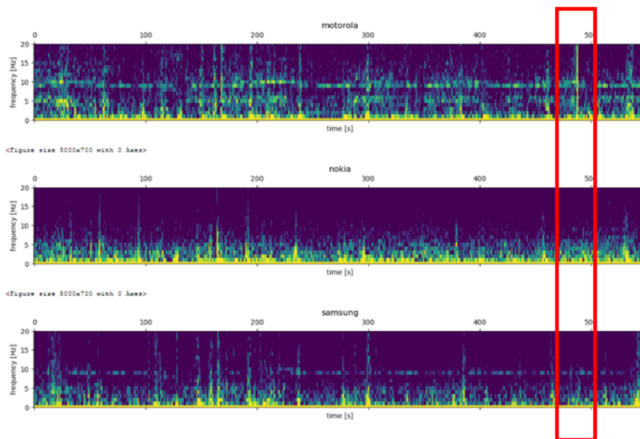
Figure 4.24: Spectrograms of the measurements on the CTO. The human-caused outlier is observable around time = 480 seconds as a bright yellow line, indicating high energy content in all frequencies.
