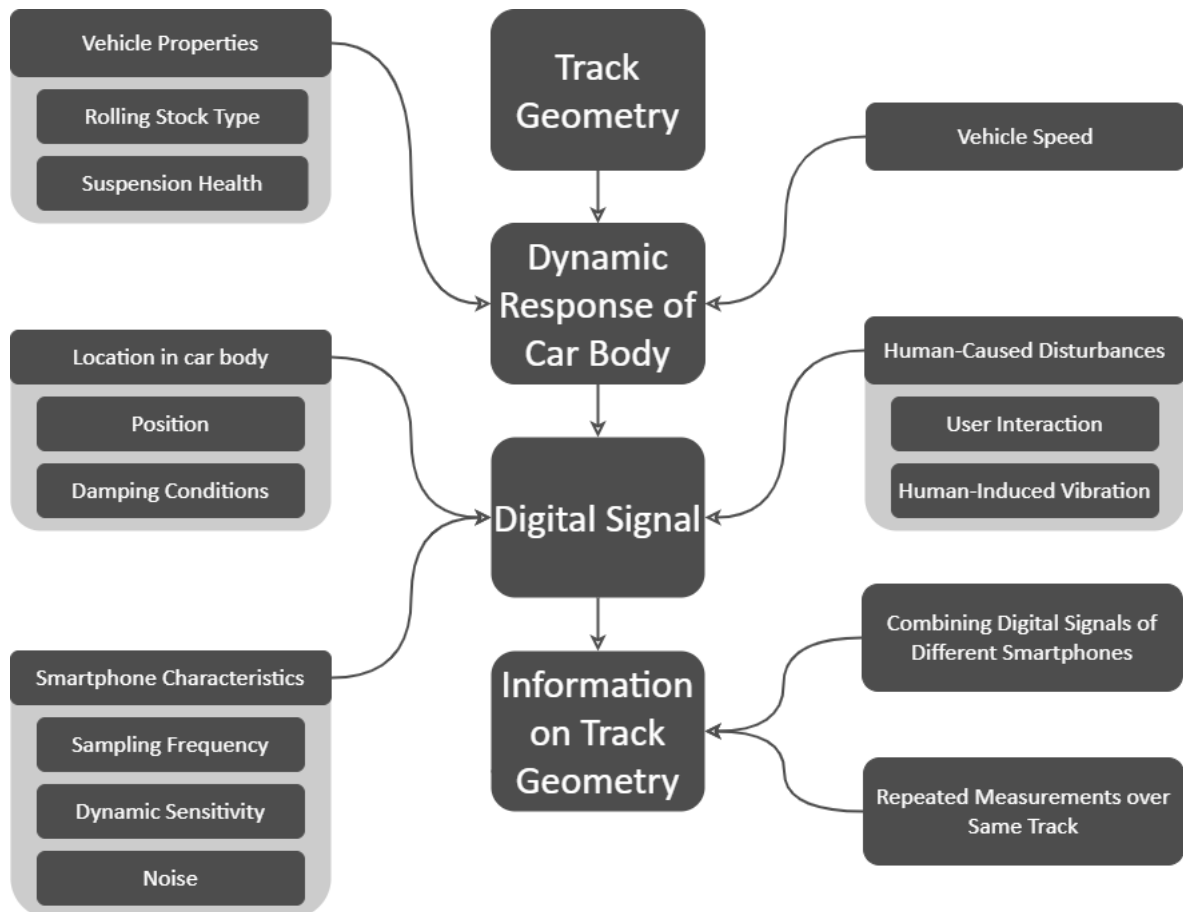
Figure 1.3: A selection of processes and variables involved in how information is obtained through smartphone accelerations.
