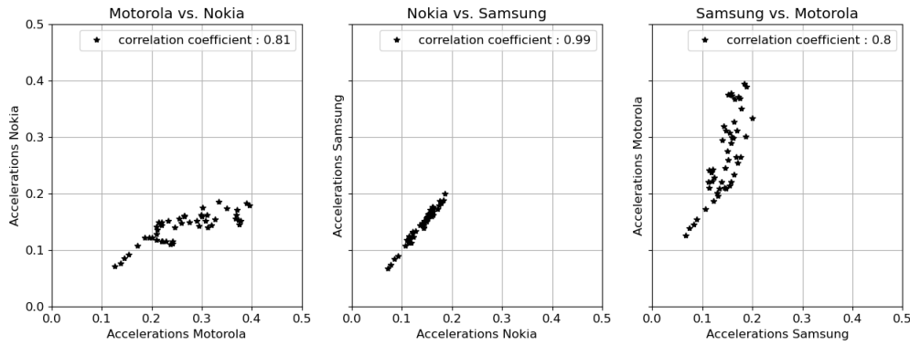
Figure 4.19: Correlation coefficients of the means found in Figure 4.18 between the different mobile phones.
