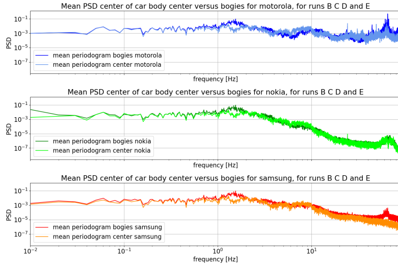
Figure 4.20: Mean periodograms of smartphones in the center of the car body and on the bogies, for all devices over measurement runs B, C, D and E.
