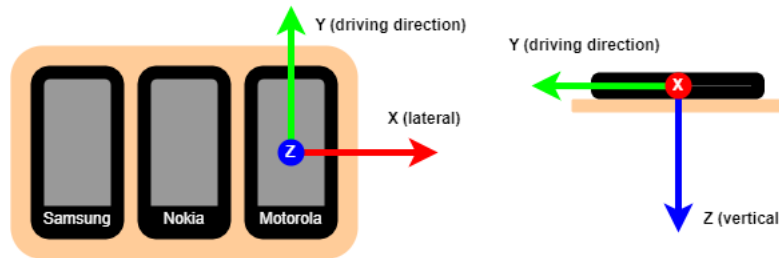
Figure 4.2: Schematic overview of the measurement boards, in relation to driving direction.
