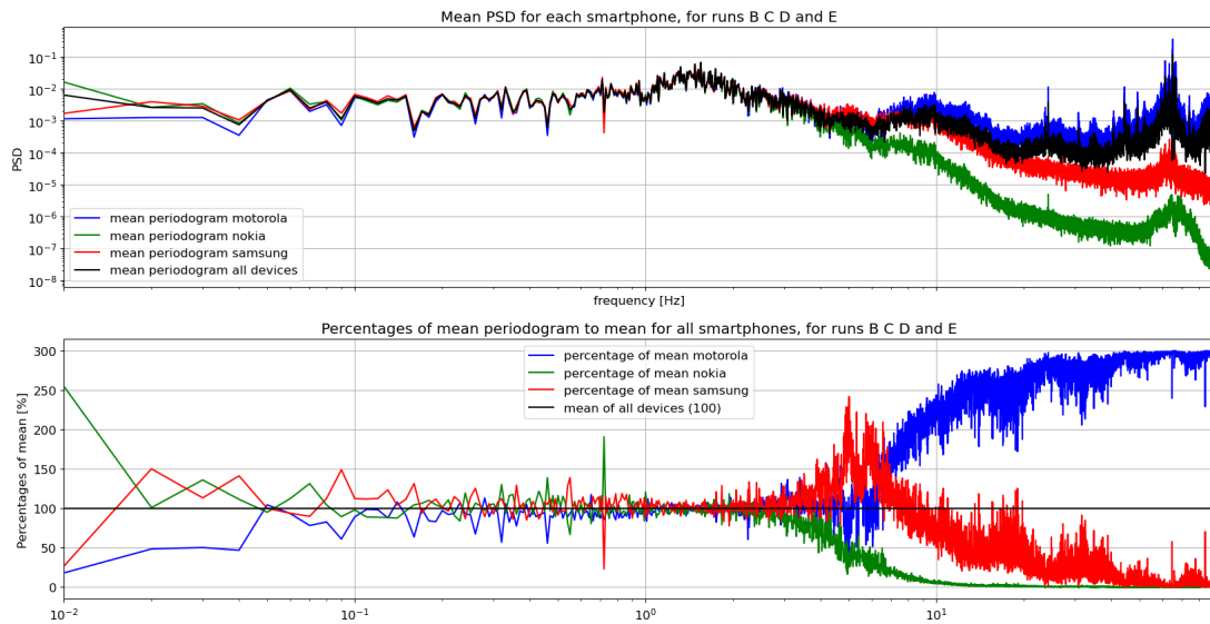
Figure 4.7: (Top) Mean periodograms for all devices over measurement runs B, C, D and E. (Bottom) Percentage of the total mean periodogram for each mean periodogram of the smartphones.
