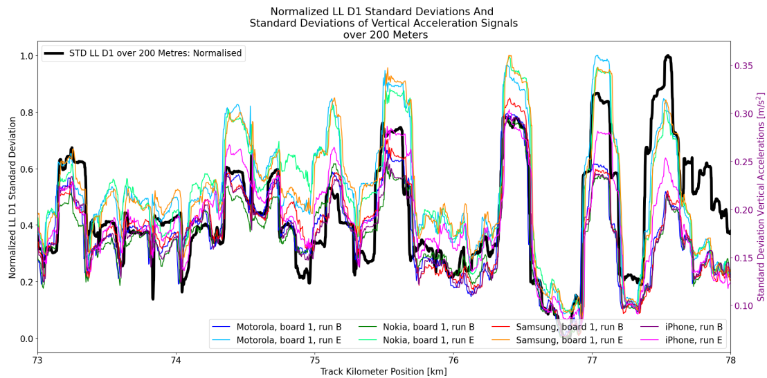
Figure 5.6: Standard deviations of the normalized track geometry and the standard deviations of the vertical acceleration signals of the smartphones. This figure includes the iPhone measurements.
