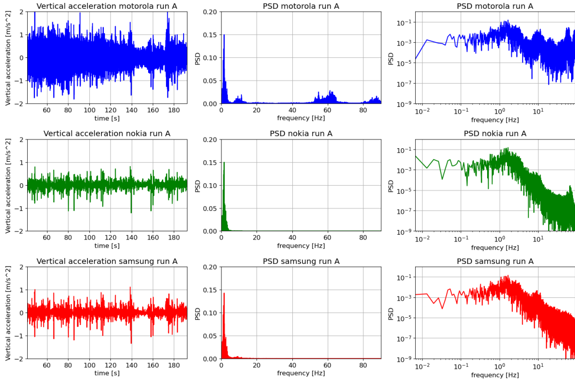
Figure 4.6: Vertical accelerations in time and frequency domain of all smartphones. The vertical accelerations are detrended by removing their mean over the entire length. The periodograms on the right are plotted on a logarithmic scale.
