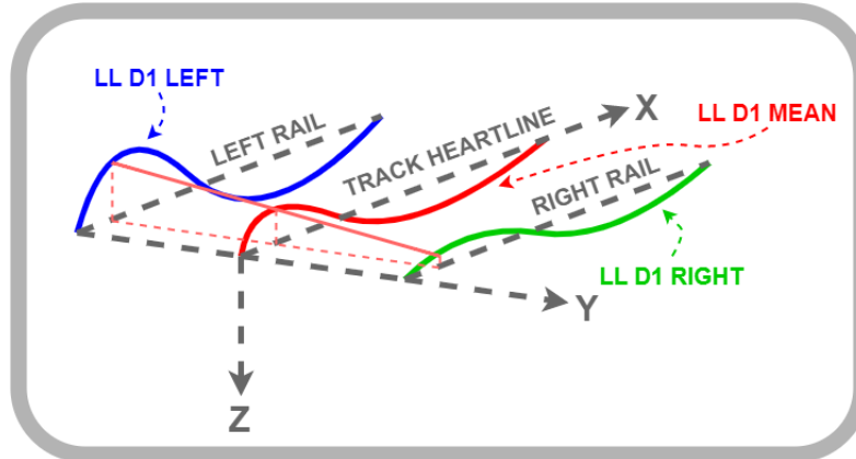
Figure 1.1: Sketch of the mean LL D1 used for track quality in this thesis. The x-, y- and z-axes correspond to the longitudinal, lateral and vertical axes respectively. The LL D1 parameters are the deviations in z-direction. The x-axis is used to denote the kilometer positions of the measured LL D1 parameter.
