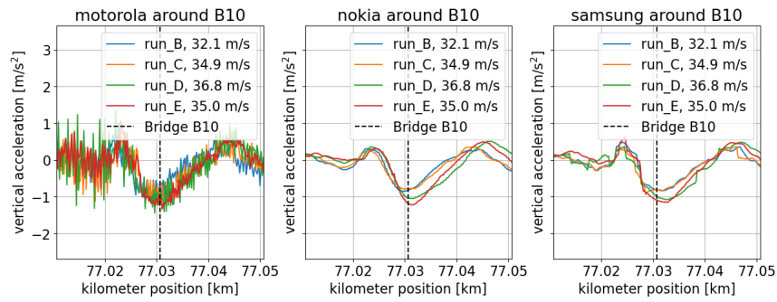
Figure 4.16: Vertical accelerations of smartphones of board 1 on different measurement runs around bridge B10.
