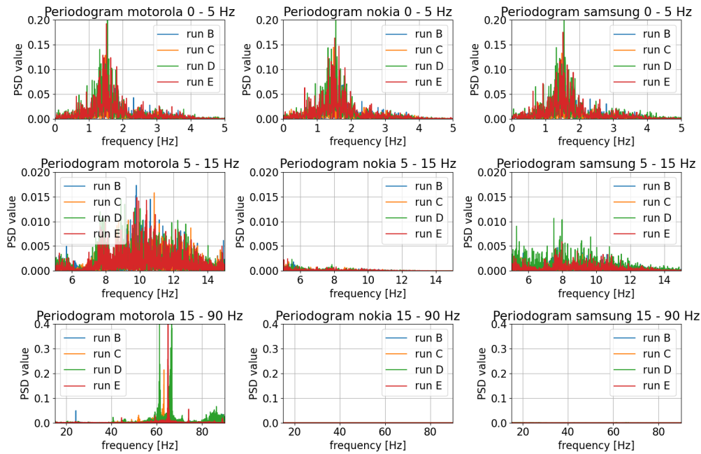
Figure 4.12: Periodograms for board 1 for each of the different runs.
