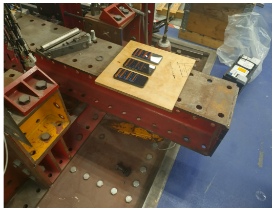
Figure 3.1: Smartphones on the structure on the rubber block.
