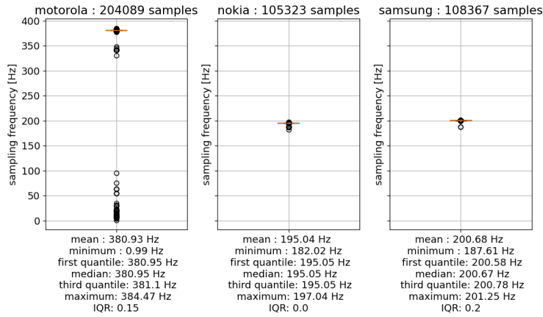
Figure 3.6: Descriptive statistics (boxplots) of the sampling frequencies over the 9 minute period
