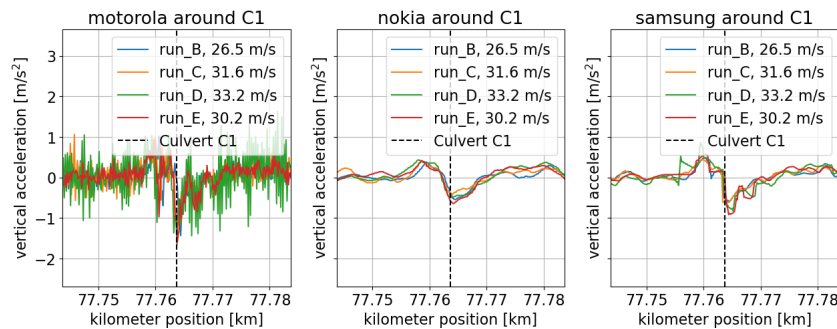
Figure 4.15: Vertical accelerations of smartphones of board 1 on different measurement runs around culvert C1.
