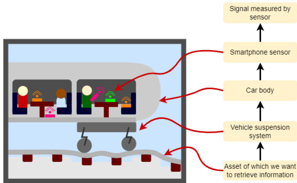
Figure 1.2: Figure of how information of the asset (track quality) travels through the vehicle and mobile phones to an acceleration signal measured by the sensor.
