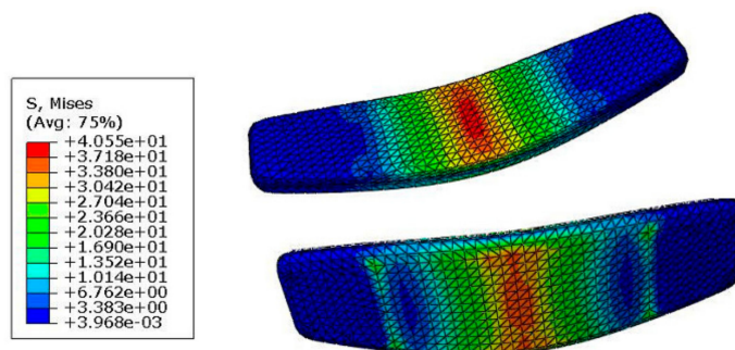
Figure 12. Von Mises stress contour of the board with the uniform honeycomb core.
