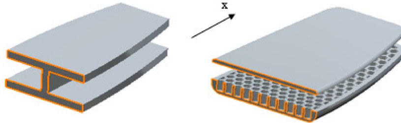
Figure 9. I-shaped beam and the board with equivalent sections shown with orange lines.
