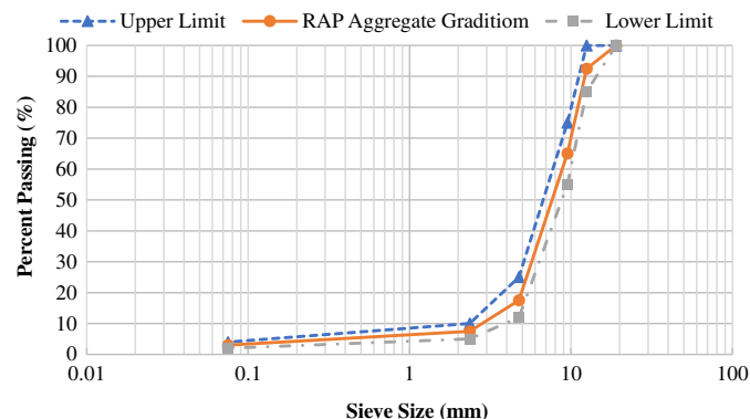
Fig. 1. The RAP aggregates' gradation.
