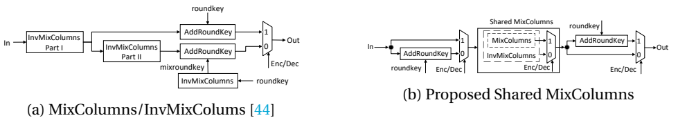
Figure 4.24: Diagram of MixColumns [44] and Proposed Shared Mixcolumns
