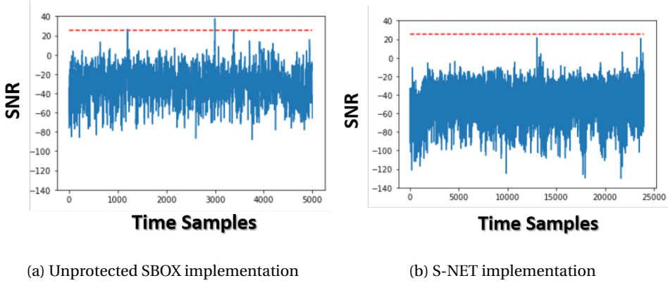
Figure 4.6: SNR analysis results
