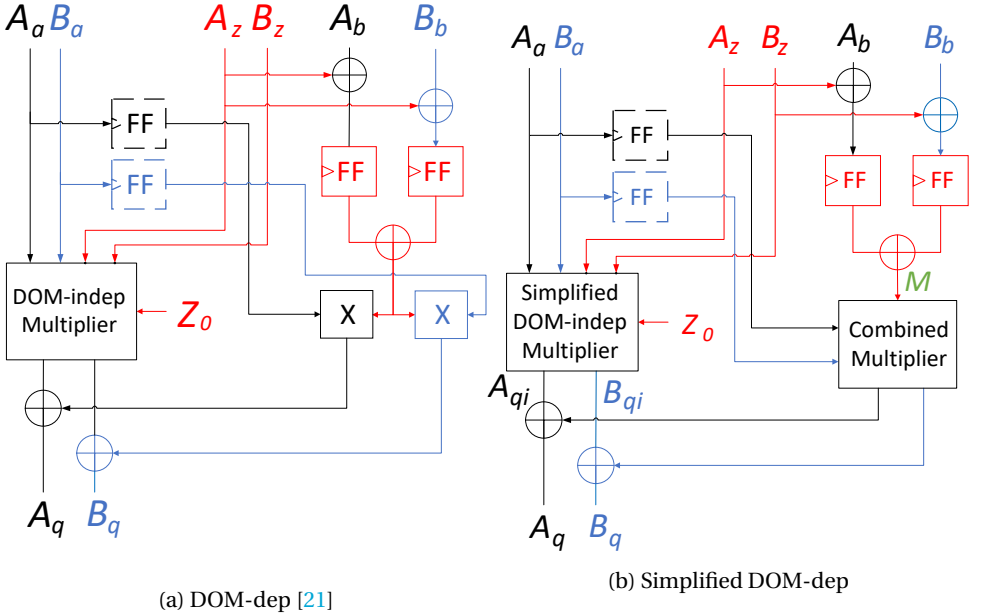
Figure 4.27: DOM-dep Multiplier [21] and Our Simplified DOM-dep Multiplier
