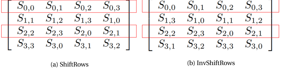
Figure 4.23: Shift Transformation of ShiftRows and InvShiftRows
