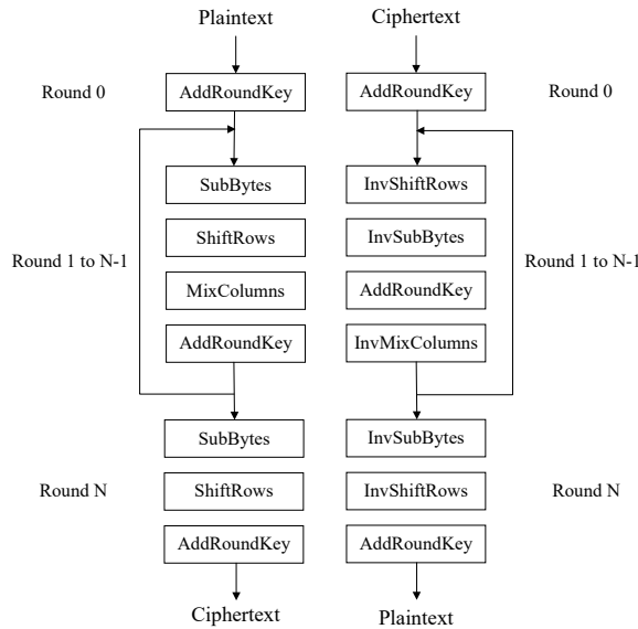
Figure 2.1: AES Encryption & Decryption Flow Diagram
