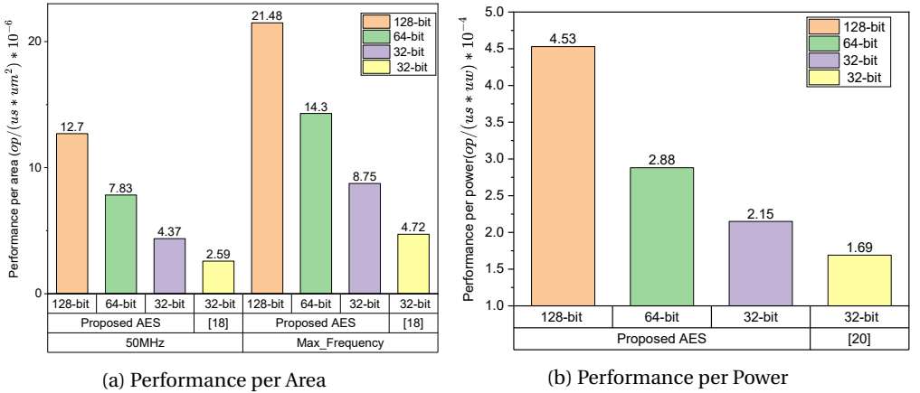
Figure 4.28: Comparison vs AES Design in [148]
