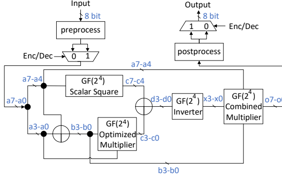
Figure 4.20: Proposed Shared SBOX
