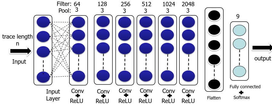
Figure 3.4: Baseline CNN with its hyper-parameters
