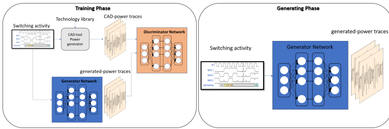
Figure 5.2: Framework Methodology
