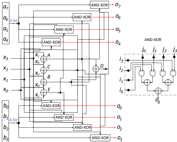
Figure 4.22: GF(2^4) Combined Multiplier
