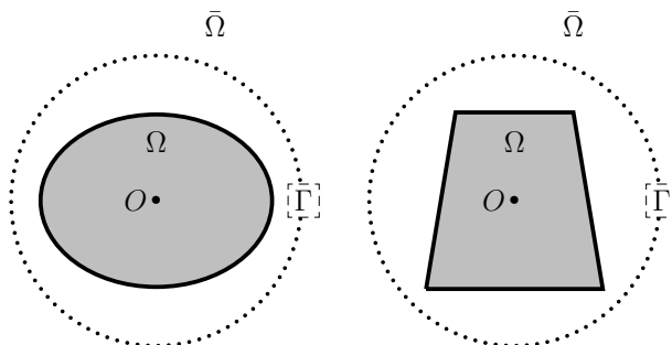
Figure 8: Sketch illustrating the possible extension of the approach detailed in this paper to elliptical (left) and trapezoidal (right) geometries.
