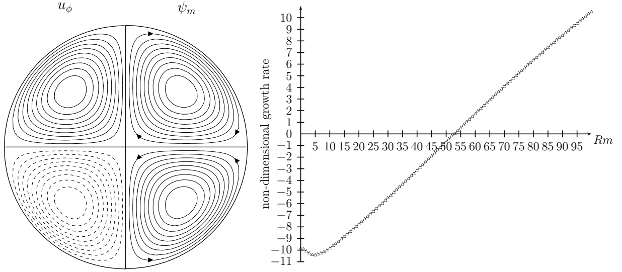
Figure 4: Left: The s2t2 flow of Dudley & James 17 . The zonal wind is denoted by u_\phi and is equatorially-antisymmetric; \psi_m is the meridional stream function, consisting of 2 counter-rotating rolls. The relative amplitude of these two flow components is measured by a dimensionless parameter \epsilon . Right: numerical estimate of the growth rate as a function of the magnetic Reynolds number Rm , for \epsilon = 0.14 . The growth rate is positive for Rm \gtrsim 53 .
