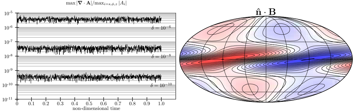
Figure 5: Left: Timeseries of the divergence level, as measured by \max |\nabla \cdot \mathbf{A}| / \max_{i=s,\phi,z} |A_i| , for different convergence tolerance level \delta in the electric potential solves. Right: the normal component of the magnetic field \hat{\mathbf{n}} \cdot \mathbf{B} on \Gamma . Scale is arbitrary (kinematic dynamo action); red (resp. blue) indicates positive (resp. negative) values.
