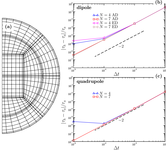
Figure 3: (a): the spectral element mesh used to compute the free magnetic decay times in a sphere, shown here for polynomial order N = 7 . (b): Relative error in free magnetic decay time as a function of timestep size, for the axial and equatorial dipole AD and ED, respectively, and for polynomial order 4 and 7. The dashed line is indicative of a second order temporal convergence. (c): same as (b) for the equatorial quadrupole EQ.
