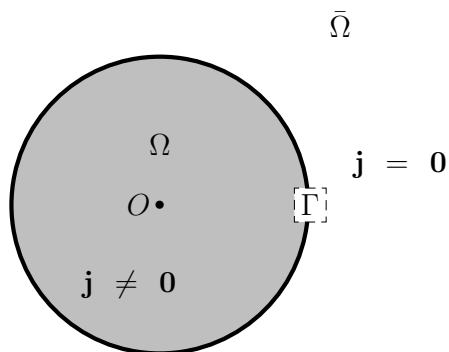
Figure 1: Notations. The computational domain \Omega (gray region) contains an electrically conducting fluid, the motion of which can generate electric currents \mathbf{j} . It is surrounded by an infinite insulating domain \bar{\Omega} . These two domains are separated by the surface \Gamma , which is assumed to be spherical when the analytical Dirichlet to Neumann operator is constructed in section 5.
