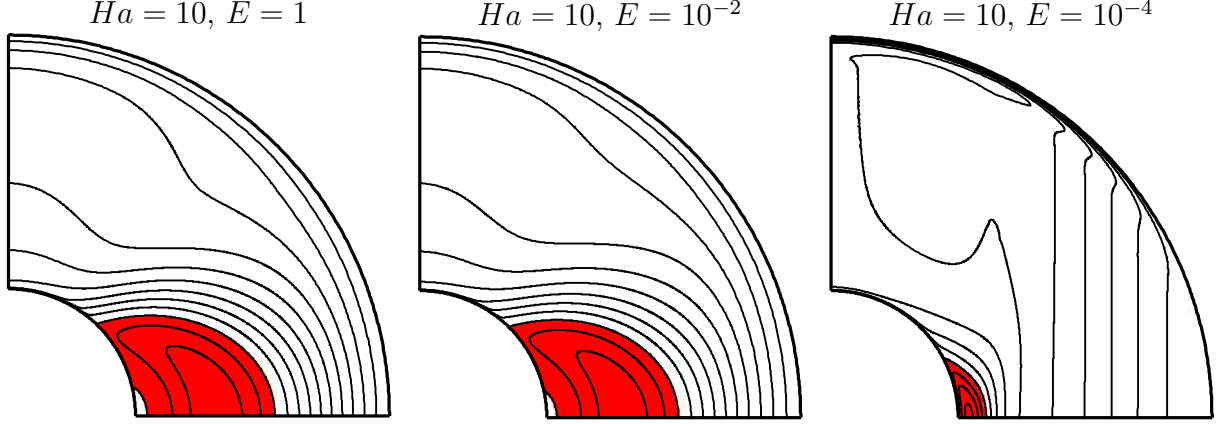
Figure 7: MHD spherical Taylor–Couette flow: maps of the normalized angular velocity u_\phi/s\Delta\omega in the semi-meridional plane. The strength of the imposed magnetic field is constant ( Ha = 10 ), as is the level of differential rotation ( Rm = 1 ). The background rotation rate increases from left to right by four orders of magnitude ( E = 1 down to E = 10^{-4} ). Contours are separated by 1/10 , and red indicates super-rotation ( u_\phi/s\Delta\omega > 1 ).
