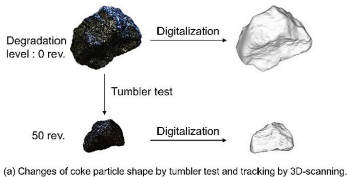
(a) Changes of coke particle shape by tumbler test and tracking by 3D-scanning.
