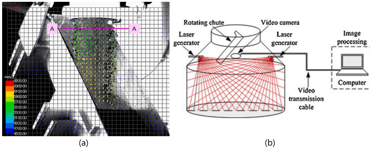
Fig. 26. (a) Example of velocity analysis by PIV [38] (b) laser grid method to capture particle trajectories [38].
