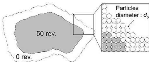
(b) Fine particles generation at 50 rev. by multi-sphere model.
