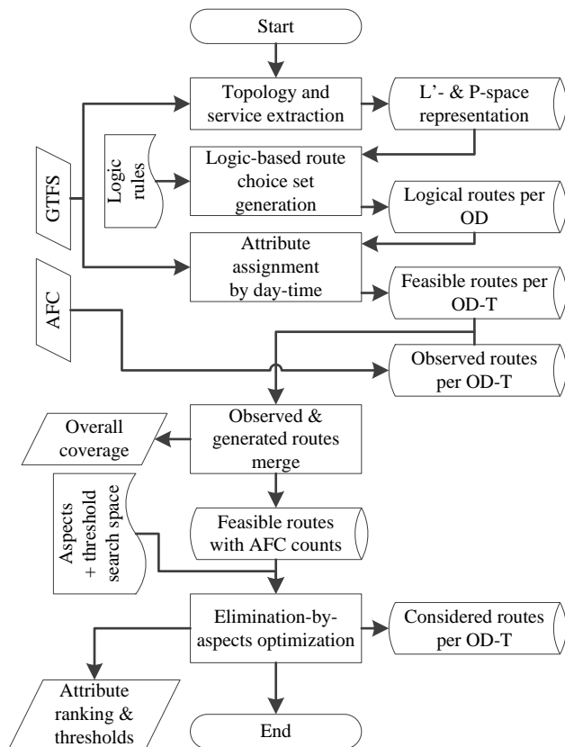
Fig. 1. Overall methodology
