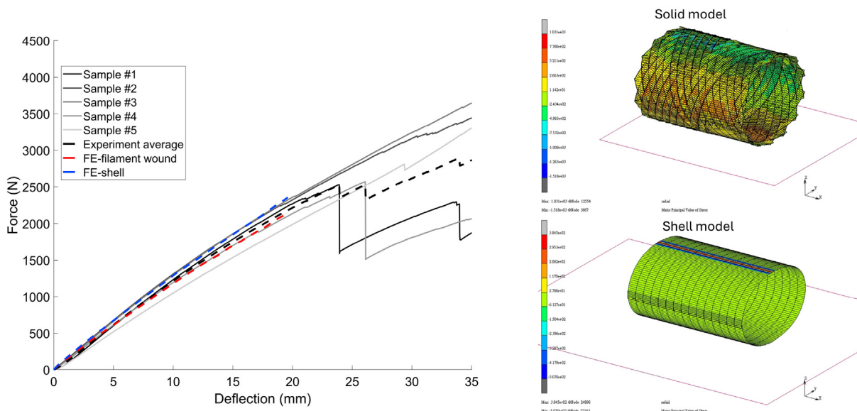
Fig. 3. Left: Force and displacement from experiment vs. FEA (shell & solid models). Right: Stress distribution for shell & solid models.
