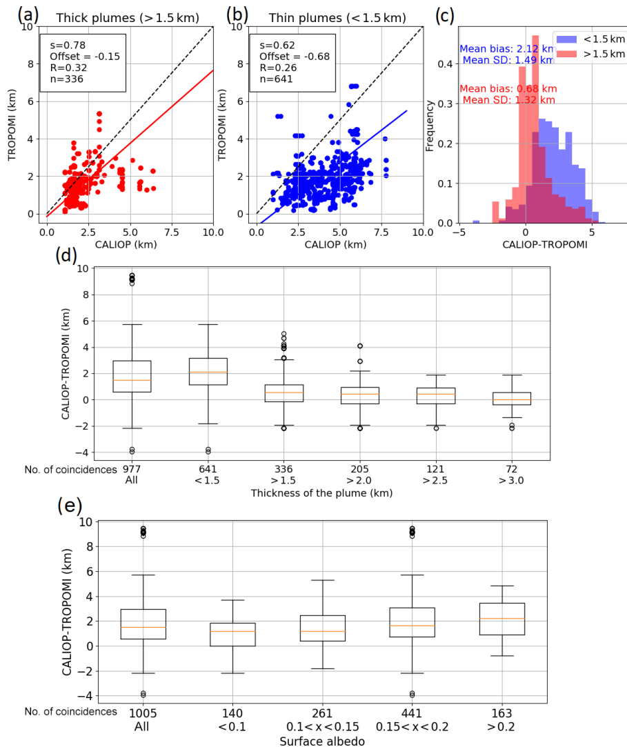
Figure 4. CALIOP–TROPOMI comparison for (a) geometrically thick plumes ( > 1.5 km) and (b) geometrically thin plumes ( < 1.5 km), together with the statistics of the line of best fit (correlation coefficient, R , slope, s , and number of observations, n ). The plume thickness is determined by the CALIOP top and base plume height. Panel (c) shows the histogram for the differences in plume height (CALIOP – TROPOMI) for thick (red) and thin (blue) plumes. Panel (d) shows the statistics for different plume thickness filters and (e) for different ranges of surface albedo.
