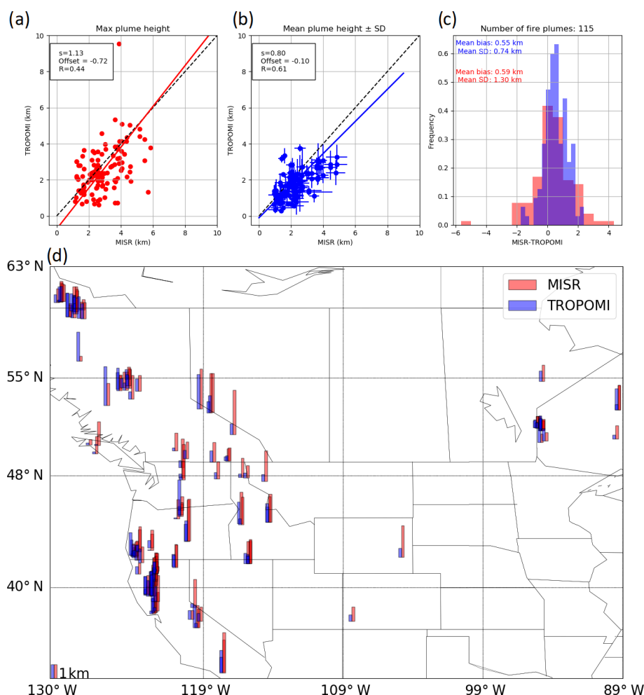
Figure 3. TROPOMI–MISR plume height comparison. In total 115 fire plumes were compared (all between June and August 2018) in terms of (a) maximum plume height and (b) mean plume height within one wildfire plume, together with the statistics of the line of best fit (correlation coefficient, R , and slope, s ). Panel (c) shows the histogram for the differences in plume height (MISR – TROPOMI) for the maximum (blue) and mean (red) plume height. (d) A map showing the regional distribution of those fires with the mean plume height (above ground level) for TROPOMI (blue; left bar) and MISR (red; right bar).
