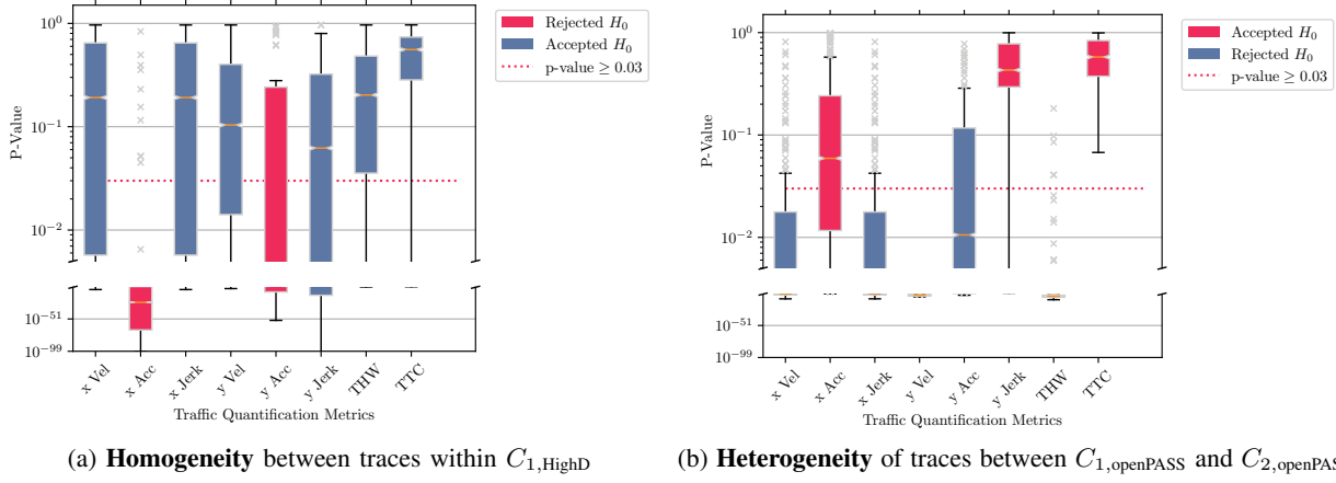
Fig. 2: Homogeneity and heterogeneity tests for traffic observation from either real-world HighD data or synthetic openPASS data.
