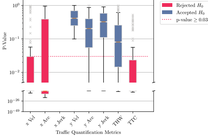
Fig. 3: The homogeneity test compares the whole traffic observation of C_{1,HighD} with its lane change sub-space. Some of the sub-space's TQMs fail the similarity test, since lane changes do not share all the same properties as the whole traffic observation.
