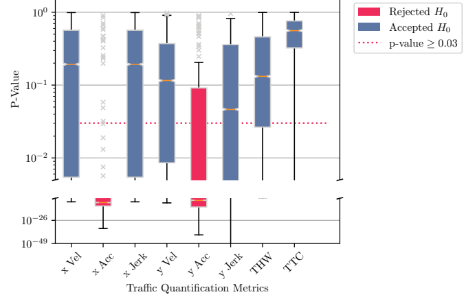
Fig. 4: Homogeneity between C_{1,HighD} and C_{1,openPASS} , expressing the quality of the simulation's recreation of a real-world traffic observation.
