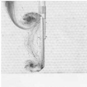
(a) h = 100 mm, t = 0.35 s. Acceleration phase.
