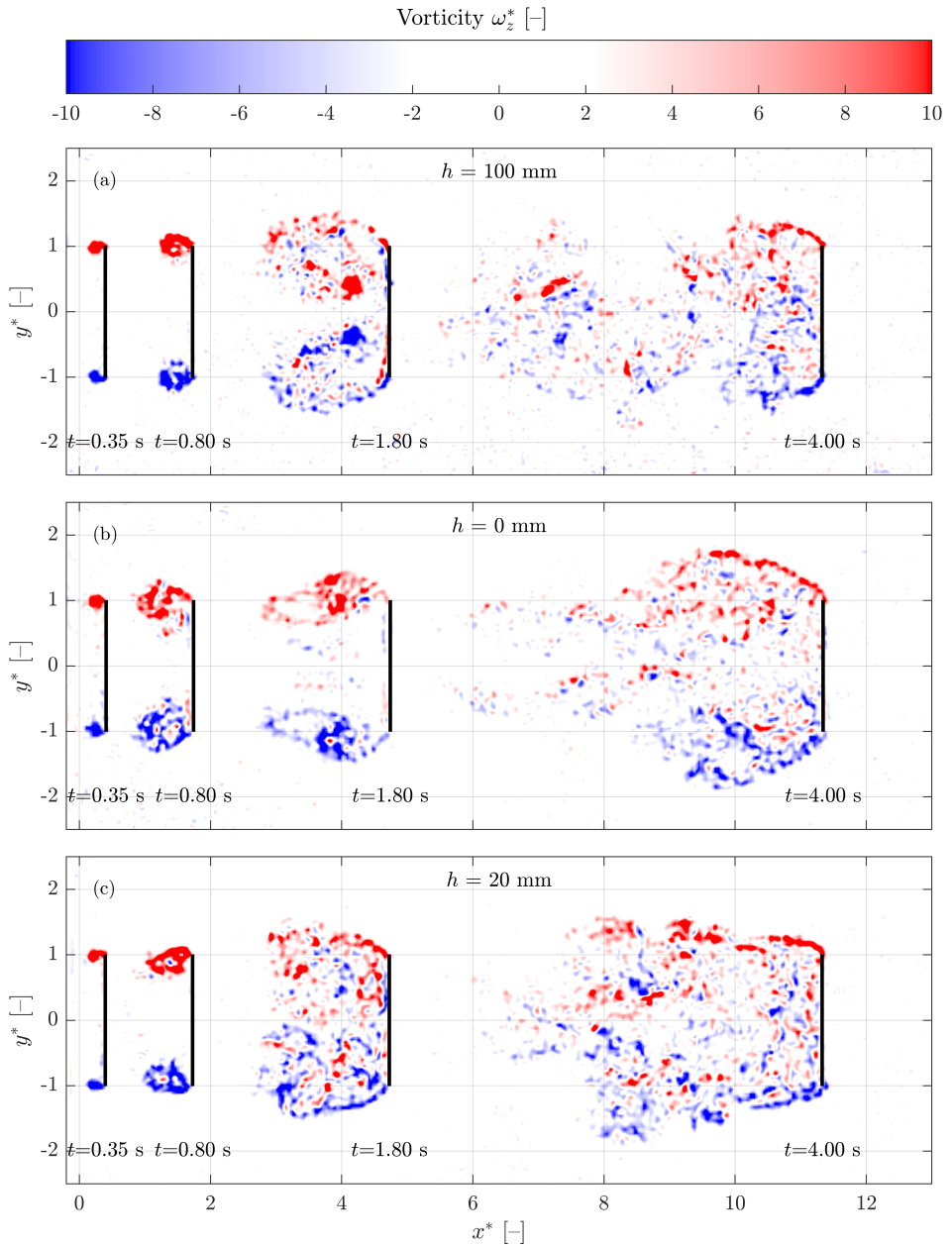
Figure 2.16: (Horizontal plane at plate half-height) Dimensionless vorticity \omega_z^* for different instances in time t at the three selected depths (a) h = 100 mm, (b) h = 0 mm, and (c) 20 mm. The plate location x^* matches the formation time t^* , i.e. x^*(t^*) = t^* .
