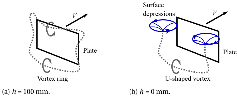
Figure 2.9: Vortex formation during the acceleration phase. In the case of h = 100 mm (a) the plate is fully submerged and a closed vortex ring is formed behind the plate. In the case of h = 0 mm (b) the top of the plate coincides with the water surface, and a closed vortex ring cannot be formed. Instead, a U-shaped vortex is formed, which attaches to the surface with both ends, creating surface depressions.
