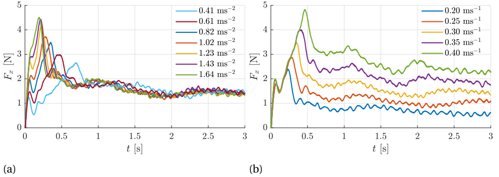
Figure 2.10: Drag force signals F_x(t) measured at plate depth h=100 mm. (a) F_x(t) for various accelerations towards a fixed plate velocity V = 0.30 \text{ ms}^{-1} . (b) F_x(t) for a fixed acceleration of a = 0.82 \text{ ms}^{-2} towards various plate velocities V .
