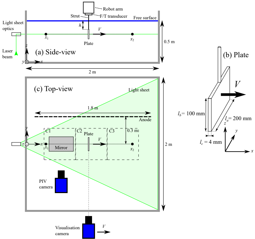
Figure 2.1: Schematic of the experimental set-up. (a) Side-view of the set-up with the robot arm holding the plate moving from x_1 to x_2 at velocity V at a distance from the free surface h . (b) Plate dimensions and orientation. (c) The top-view showing the horizontal light sheet used for particle image velocimetry (PIV) that crosses the plate at half-height. The PIV camera images the field of view via a mirror. Both the camera and mirror are positioned underneath the tank and are moved to different position for each field of view (C1, C2, C3). Also, the anode and the camera moving with the plate for the flow visualisations are shown.
