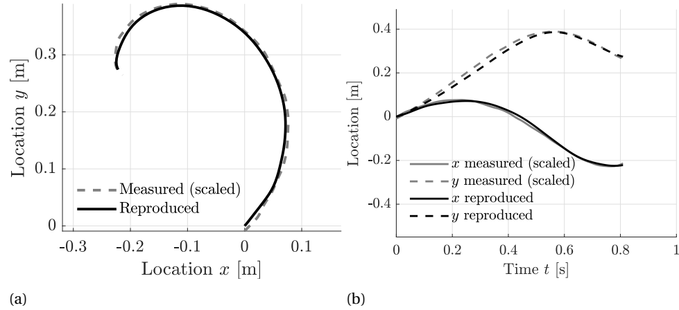
Figure 3.7: Comparison of the measured (and scaled) path of the oar blade tip (dashed grey line) and the path of the oar blade tip reproduced by the robot (solid black line). (a) The path of the blade tip in the x - y plane. (b) The coordinates x and y of the blade tip as a function of time t .
