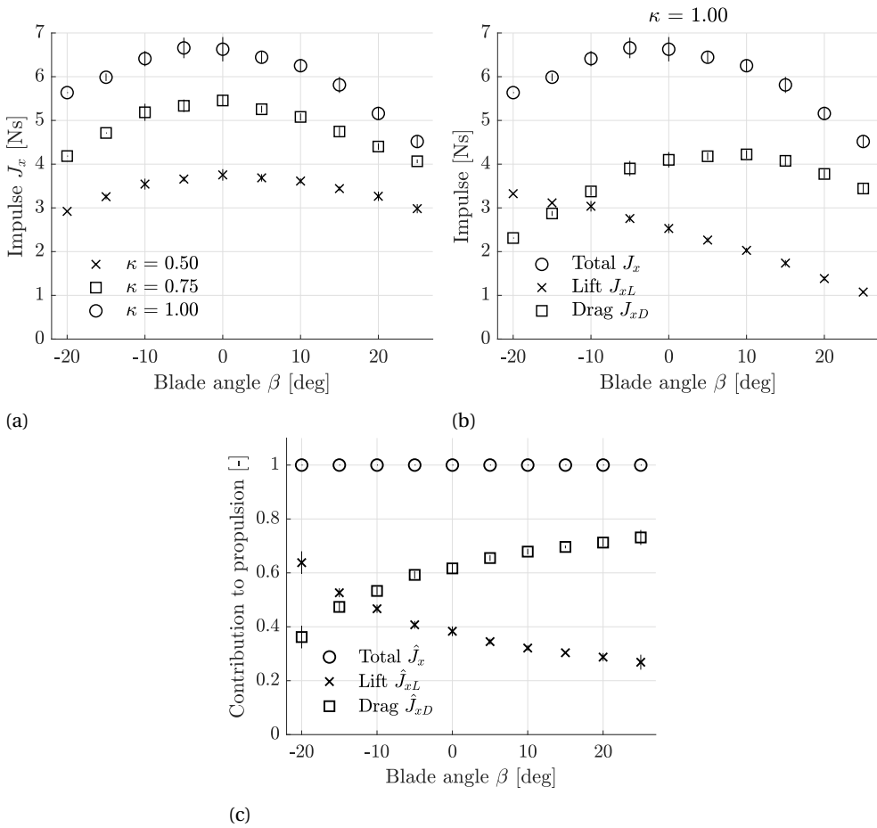
Figure 3.17: (a) The effectiveness J_x , i.e. the impulse generated in x -direction as a function of the blade angle \beta for different velocity scaling factors \kappa = 0.50, 0.75, and 1.00 . (b) The contribution of the lift J_{xL} and drag J_{xD} to the total propulsive impulse J_x as a function of blade angle for \kappa = 1.00 . (c) The relative contribution of the lift and drag to propulsion as a function of \beta for all velocity scaling factors \kappa . (all) The vertical bar in each marker indicates the standard deviation of the measurements.
