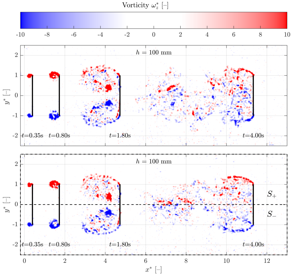
Figure 2.17: (Horizontal plane at plate half-height) Dimensionless vorticity \omega_z^* for different instances in time t at a selected depth of h = 100 \text{ mm} . The flow behaviour appears to be very similar for both realisations. Only in the steady phase t = 4.00 \text{ s} the tail of the wake sweeps up in one realisation (top figure) and down in the other (bottom figure) which matches the characteristic oscillating wake as was already observed by Fage & Johansen [13]. The dashed line around the outer border shows the area of integration S for which the circulation is obtained. The symmetry line through y^* = 0 is also marked and shows the dividing line between integration surfaces S_- and S_+ .
