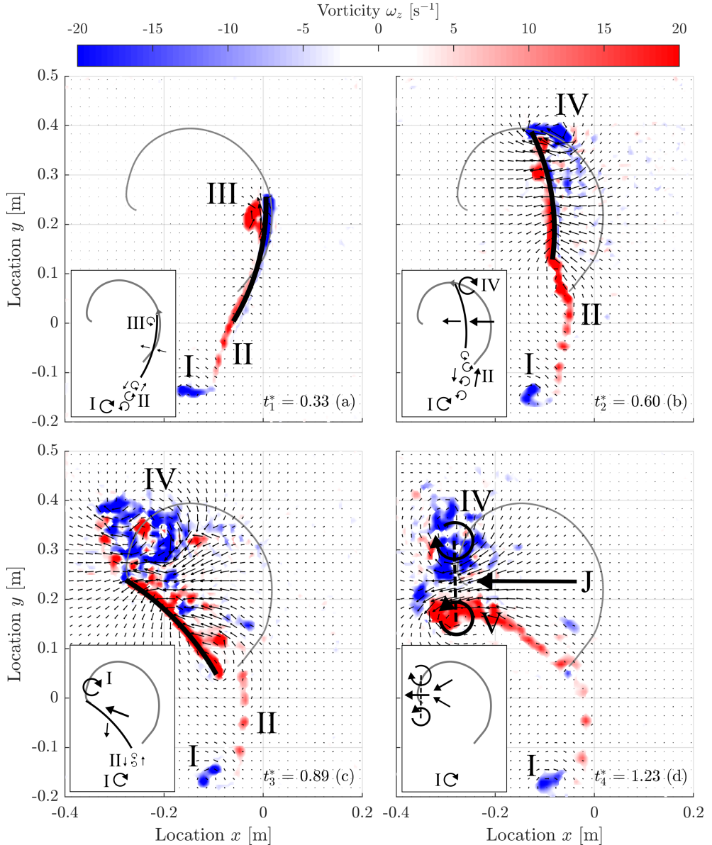
Figure 3.20: Snapshots of the velocity field (black arrows) and the vorticity (contours) for the selected times t_1^* to t_4^* as indicated in figure 3.19. The snapshots are taken at (a) the start of the drive phase t_1^* = 0.33 , (b) in the middle of the drive phase t_2^* = 0.60 , (c) just before the release t_3^* = 0.89 and (d) just after the release t_4^* = 1.23 . The blade and blade path are shown as black and grey curve, respectively. In each snapshot an inset sketches the flow. A straight arrow indicates the flow direction and relative magnitude and the circular arrows indicate vortical structures. Roman numeral I indicates a starting vortex, II a vortex sheet, and III and IV a leading edge vortex. In (d) a vortex pair IV-V and the impulse vector \vec{J} are shown. The trailing-edge vortex layer rolls up in a vortex with opposite circulation than the LEV, so that they form a vortex pair that propels itself to the left. A jet-type of flow is generated more or less in negative x -direction, an indication of propulsion.
