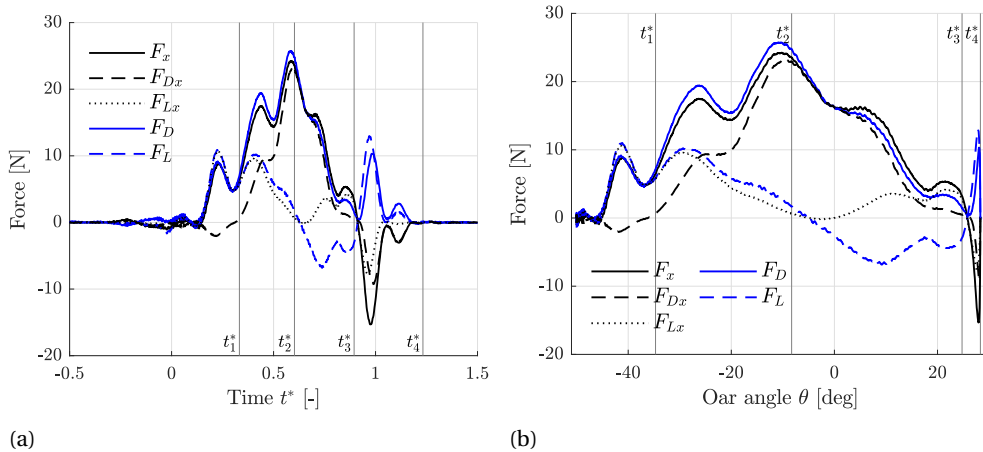
Figure 3.12: The propulsive force F_x is composed of the propulsive part F_{Dx} due to drag F_D and the propulsive part F_{Lx} due to lift F_L as a function of (a) dimensionless time t^* and (b) the oar angle \theta for \kappa = 1.00 . The lift is positively contributing to propulsion up to the start of the release at \theta \approx 25^\circ . In both figures the vertical lines indicate the times of the flow field snapshots shown in figure 3.14. Dimensionless time t_1^* = 0.33 is roughly in the middle of the lift phase, t_2^* = 0.60 is at maximum propulsion, t_3^* = 0.89 is at a minimum drag just before the release and t_4^* = 1.23 is just after the release.
