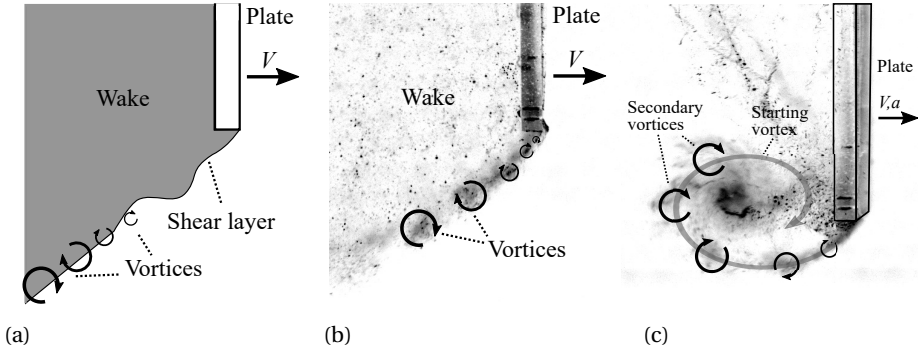
Figure 2.7: (Side view) (a) The flow separates at the plate edge. At some distance from the plate vortices are formed due to the Kelvin-Helmholtz-like instability in the shear layer coming from the plate edge. (b) At constant velocity small vortices are generated in the shear layer and shed into the wake, similar to the observations by Prandtl [31]. (c) The shear layer with the smaller secondary vortices rolls up during the acceleration phase to form the large starting vortex in a very similar way as was observed by Lian & Huang [24].
