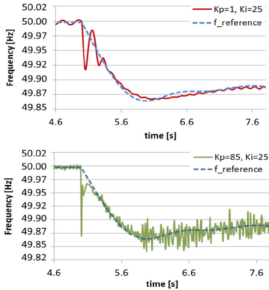
Fig. 12 Impact of the setting of K_p on dynamics of the PLL
