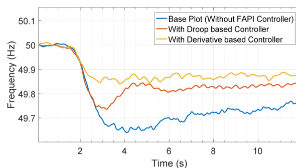
Fig. 19 Frequency response due to load increase at Bus 8. (comparisons with different FAPI controllers)
