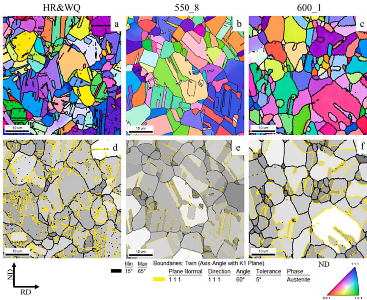
Fig. 1. ND IPF maps of the a) HR&WQ, b) 550_8, and c) 600_1 sample. GAIQ maps with \Sigma 3 twin boundaries plotted in yellow for the d) HR&WQ, e) 550_8, and f) 600_1 sample. (For interpretation of the references to colour in this figure legend, the reader is referred to the web version of this article.)
