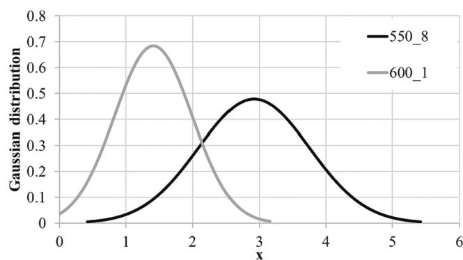
Fig. 7. The gaussian distribution plotted based on the diameter of the \kappa -carbides for the 550_8 and 600_1 samples.
