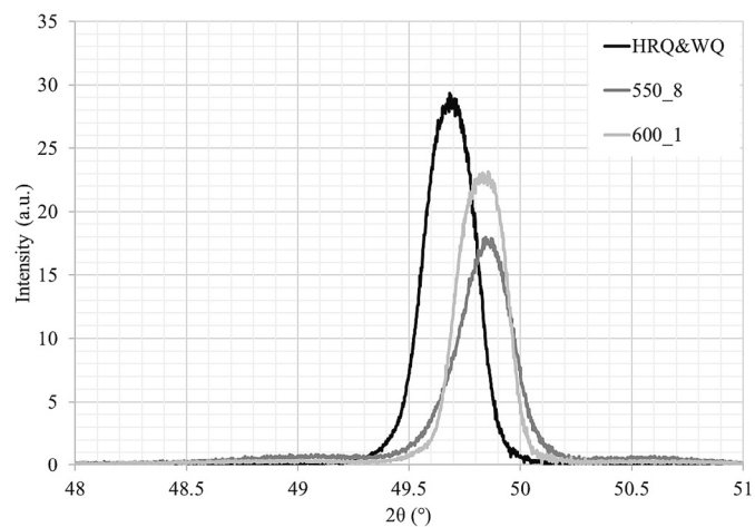
Fig. 8. XRD analysis of the HR&WQ, 550_8, and 600_1 sample at a 2\theta range between 48 and 51°.
