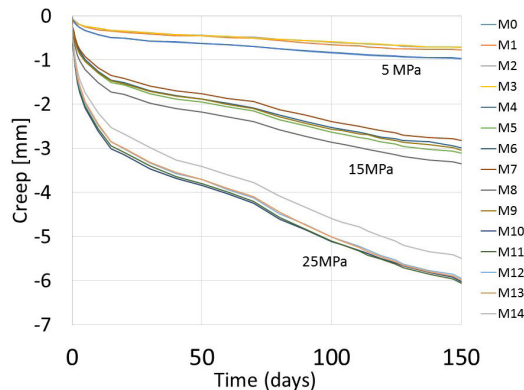
FIGURE 5.10 Creep curves at three stress levels 5, 15 and 25 MPa in three-point bending tests.
