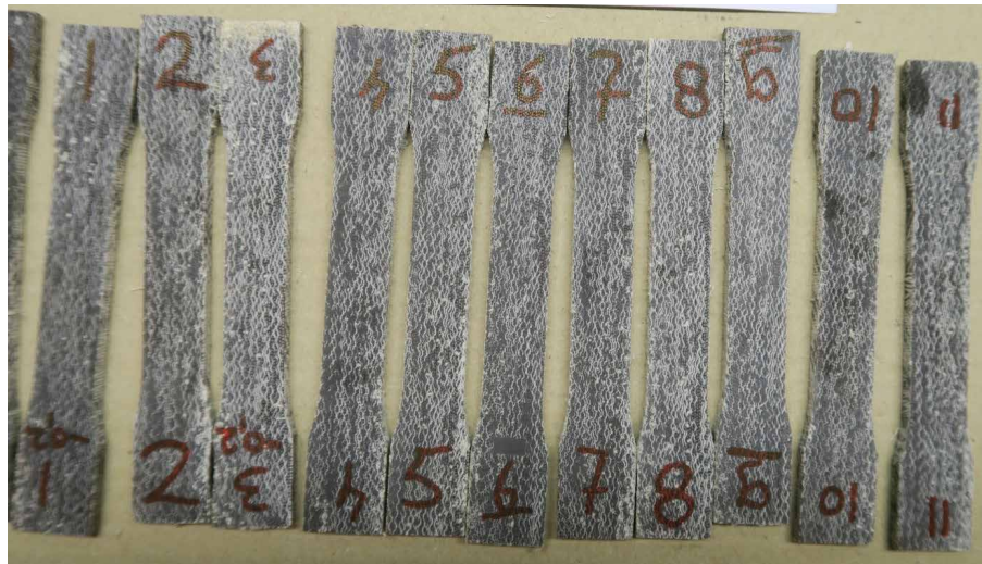
FIGURE 5.7 Milled test samples from 1:1 model and Tension test with optical strain measurement. R. Blok, J. Smits et al., Eindhoven University of Technology & Delft University of Technology, (2017).
