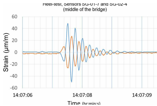
FIGURE 5.22 Strain results versus time of Sensors 1-7 and 2-4 showing eigenfrequency and damping.
