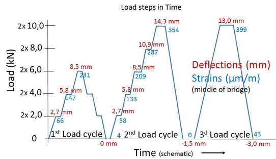
FIGURE 5.24 Three load cycles during the test on 17-08-2018 showing applied load, max strain in middle and maximum measured vertical deflection.
