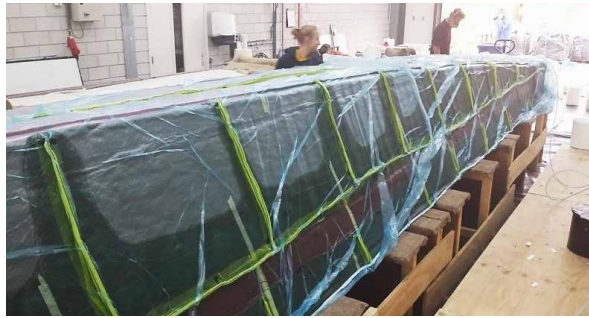
FIGURE 5.16 Bridge beam during Vacuum injection. R. Blok, J. Smits et al., Eindhoven University of Technology & Delft University of Technology, (2017).
