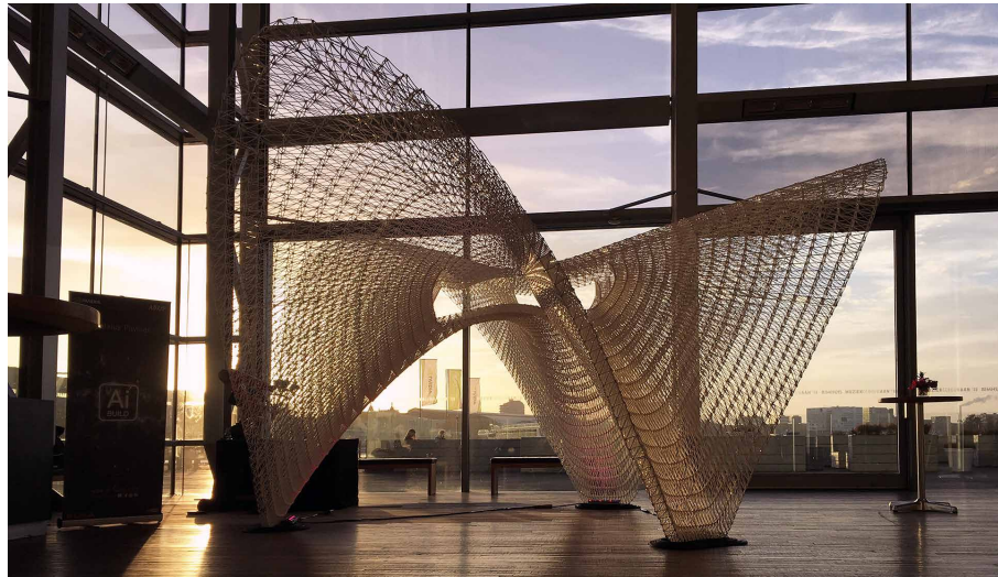
FIGURE 3.11 3D printed Daedalus Pavilion at the GPU. Photo from https://ai-build.com/daedalus.html , visited on 27/2/2019.
