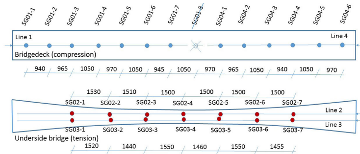
FIGURE 5.12 Location of Sensors. Line SG-01 and SG-04 are mainly compression (in bridge deck). Line SG-02 and SG-03 are mainly tension (under-side bridge). R. Blok, J. Smits et al., Eindhoven University of Technology & Delft University of Technology, (2017).
