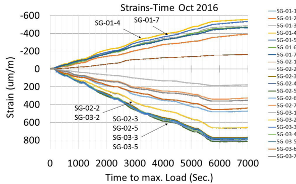
FIGURE 5.21 Strain development versus time during loading; Lines 2 and 3 are positive strains in tension (underside bridge-beam) line 1 shows negative strains in compression (in bridge deck).
