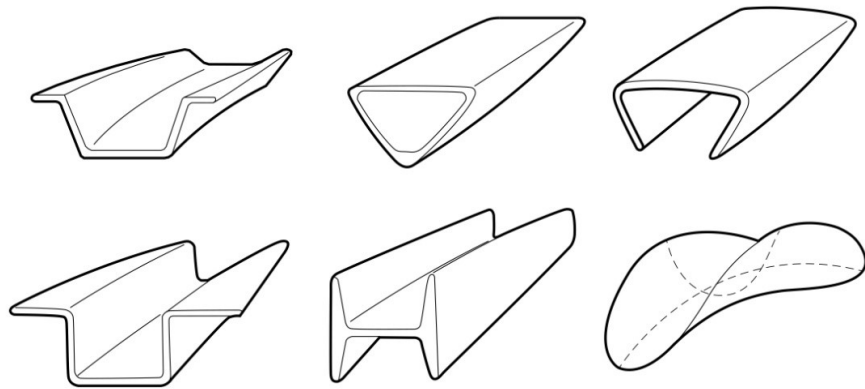
FIGURE 5.5 Workshop output on variable bridge cross-sections. R. Blok, J. Smits et al., Eindhoven University of Technology & Delft University of Technology, (2017).
