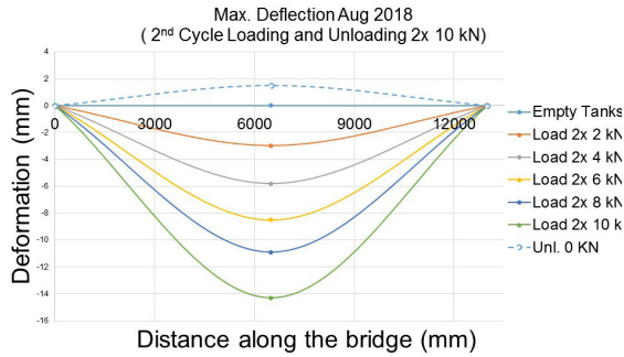
FIGURE 5.28 Measured deflections (in middle of the bridge) during second loading (10 kN) and unloading cycle.
