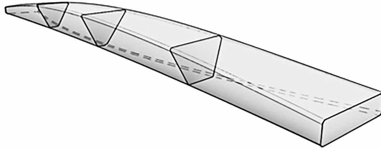
FIGURE 5.6 Different sizes and shapes of mid-span sections evaluated. R. Blok, J. Smits et al., Eindhoven University of Technology & Delft University of Technology, (2017).
