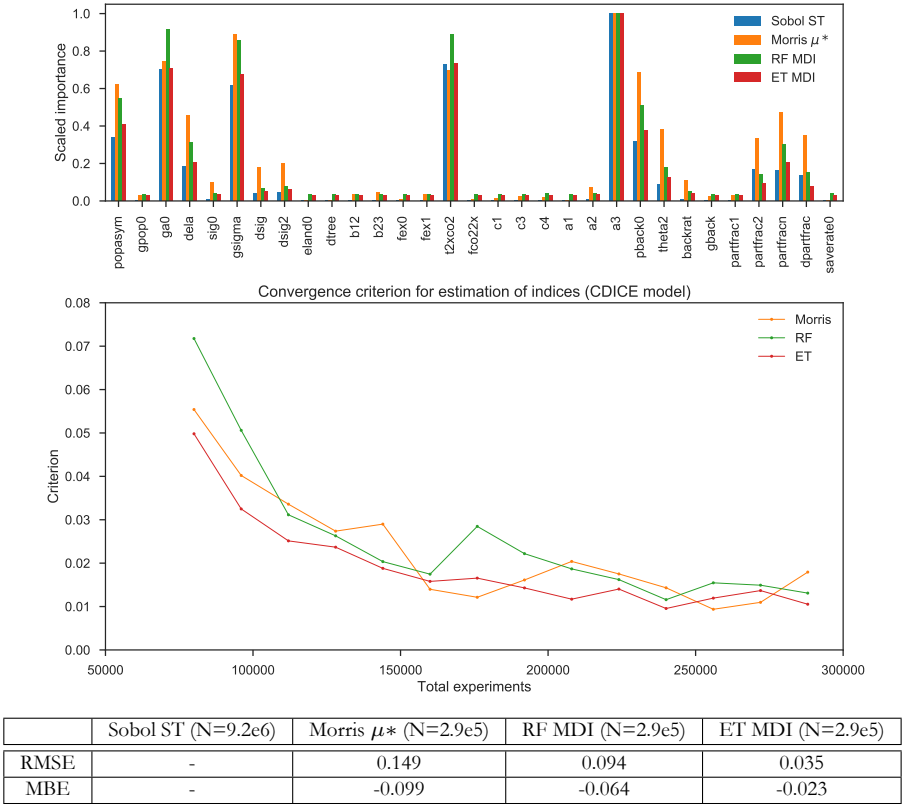
Figure A.3: Scaled variable importances and error measures for CDICE model.
