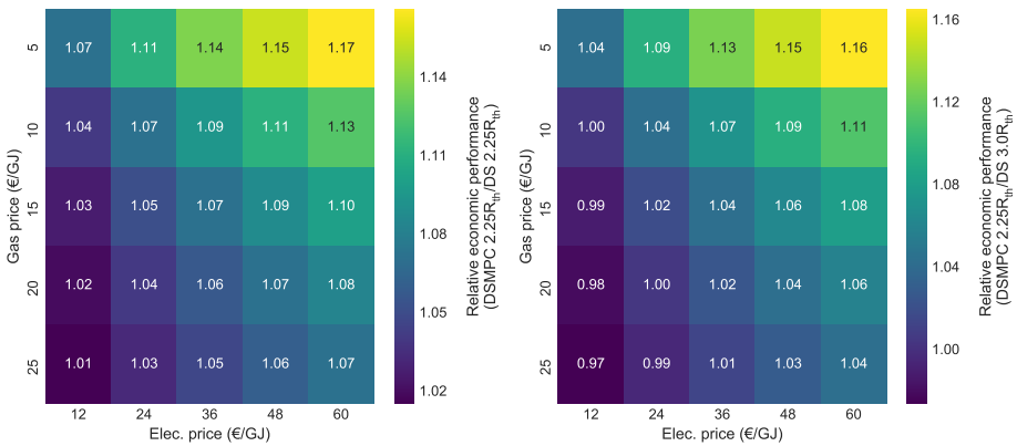
Figure 7.11: Relative economic performance across different control/layout combinations. Left panel: DSMPC compared to DS, for Scenario 3 (2.25 R_{th} ). Right panel: DSMPC for Scenario 3, compared to DS for Scenario 1.
