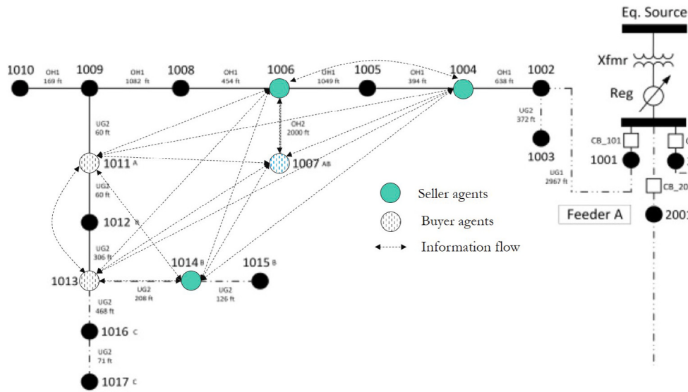
Fig. 6. Distribution feeder [68].
