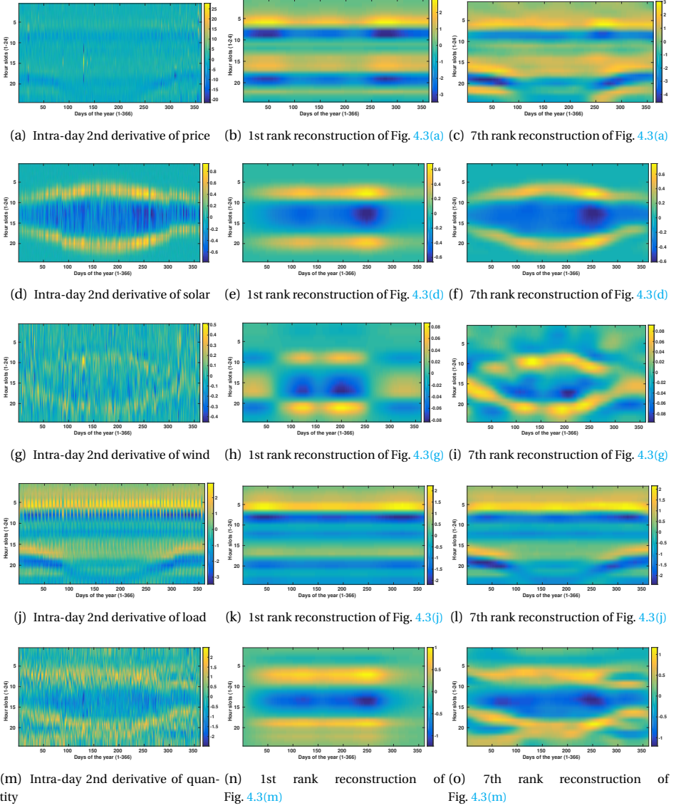
Figure 4.3: Left: The intra-day 2nd derivative of the daily profiles in 2016, for (top to bottom) price, solar and wind feed-in, load and traded quantity. The underlying trends are magnified using rank-1 (middle) and rank-7 (right) reconstruction.
