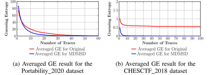
Fig. 9. Results for the two datasets considering portability.
