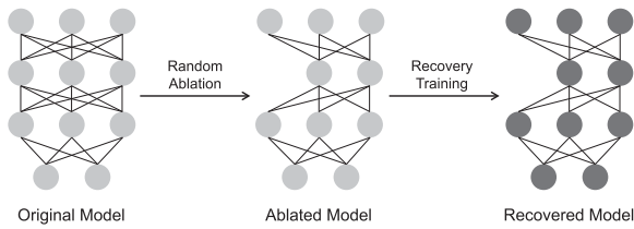
Fig. 1. A demonstration of the proposed ablation method.
