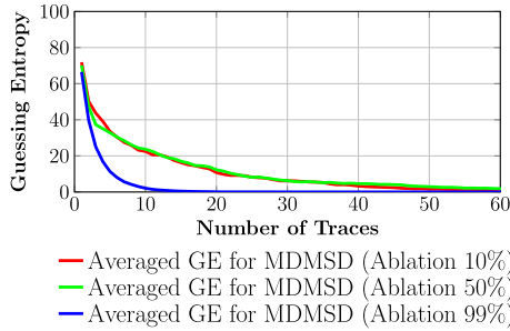
Fig. 4. Results of averaged GE for (B1_K1)–(B2_K2) and (B1_K1)–(B4_K3).
