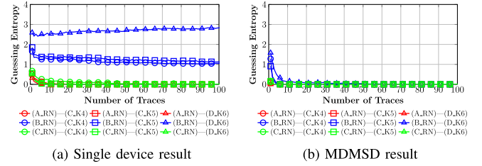
Fig. 8. Results for the CHESCTF_2018 dataset.
