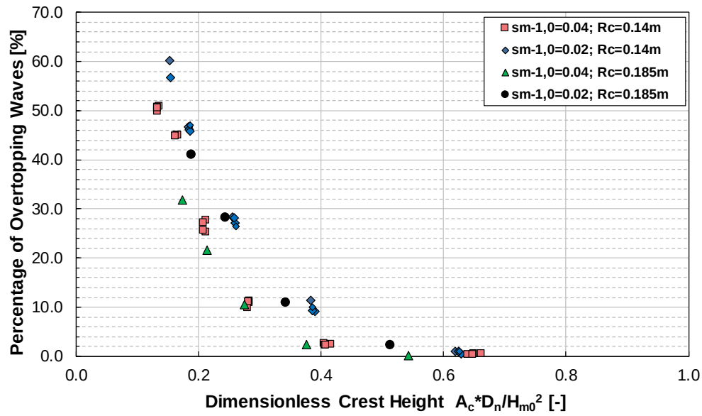
Figure 11: Percentage of wave overtopping as a function of dimensionless crest freeboard
