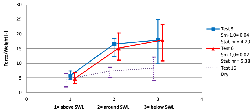
Figure 14: Overview of average interlocking degree for \phi=0.63
