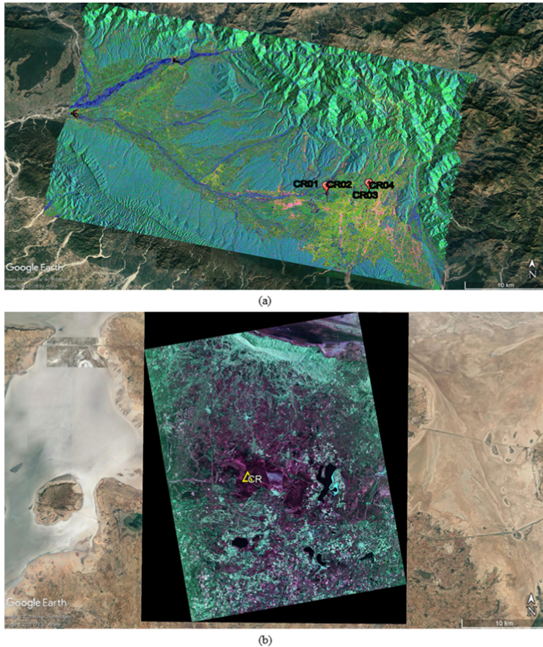
Fig. 4. Location of corner reflectors in (a) Freeman-Durden decomposition-based false-color composite of RADARSAT-2 data for Dehradun, India (b) Cloude's three-component decomposition-based false-color composite of RISAT-1 data for Desalpar, Rann of Kutch, India.
