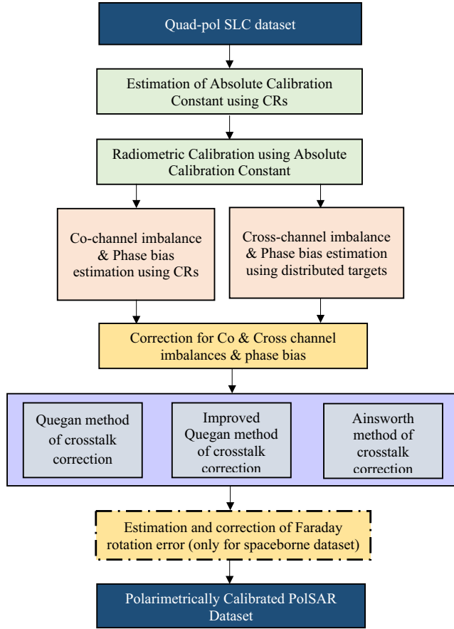
Fig. 8. Methodology flowchart for polarimetric calibration of Quad-pol datasets.
