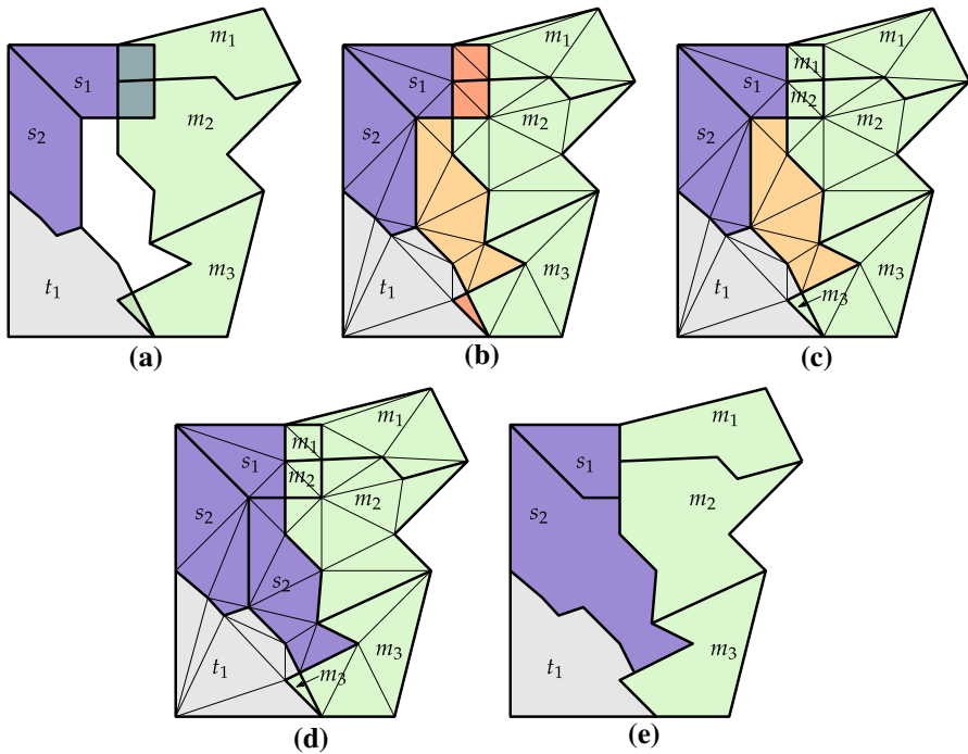
Fig. 7 a Three datasets ( S purple; T grey; M green), having, respectively, 2, 1 and 3 polygons, need to be aligned. b The CDT of the datasets with problematic regions highlighted (red overlaps; orange gaps). c Overlaps are repaired with the random neighbour method. d Holes with the same method. e Resulting aligned datasets (colour figure online)
