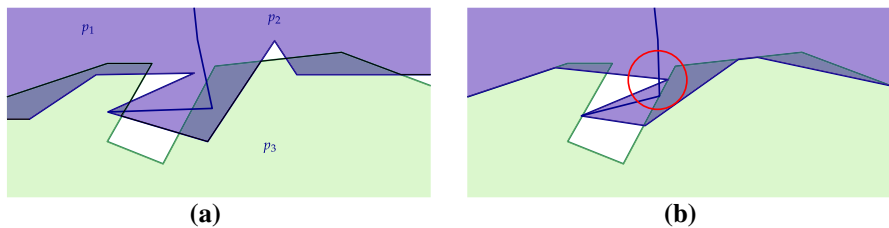
Fig. 3 a One dataset to be conflated is formed by two polygons ( p_1 and p_2 ). b Snapping the vertices of the blue dataset to the closest primitives in the green dataset introduces topological errors and intersections (in the red circle ) (colour figure online)
