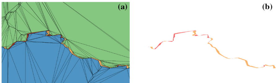
Fig. 13 For the datasets in Fig. 1a, a labelled triangulation of the datasets, and b errors as polygons. For both: red overlap and orange gap (colour figure online)
