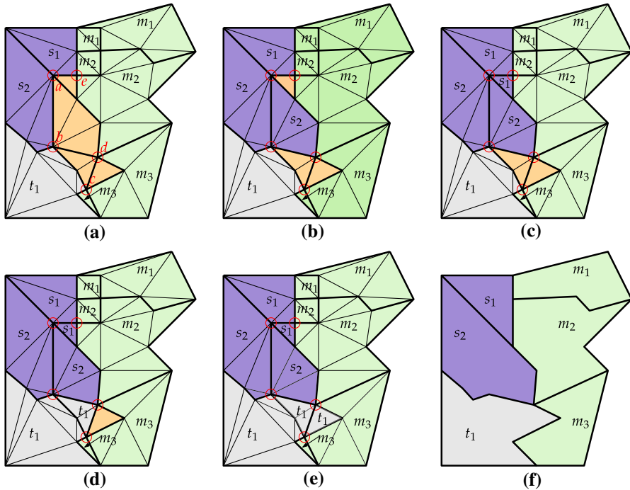
Fig. 8 The same three input datasets as in Fig. 7. The overlapping regions have already been repaired. a five split vertices are identified ( a–e ), and three extra constrained edges are inserted in the CDT ( bd , cd and the one incident to a ), separating the gap region into four sub-regions. b The sub-region adjacent to s_2 is relabelled. c The sub-region adjacent to s_1 is relabelled. d The sub-region adjacent to t_1 is relabelled. e The last sub-region is relabelled (to t_1 ). f The resulting aligned datasets
