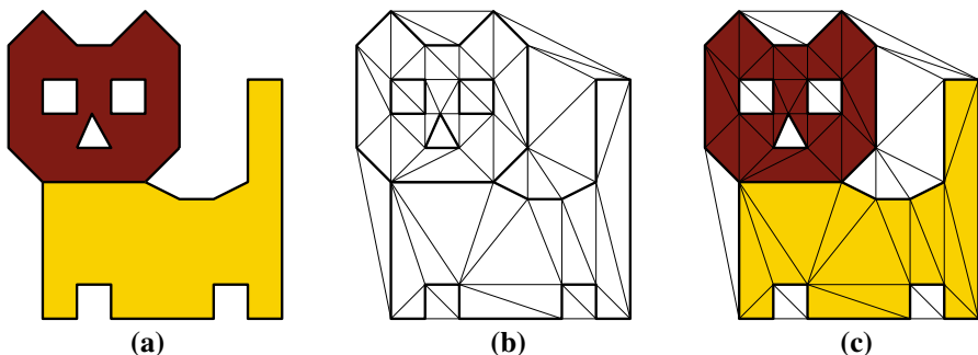
Fig. 5 a Two adjacent polygons, one of them containing 3 holes. b The constrained Delaunay triangulation of the segments of these two polygons. c From the CT, it is possible to obtain the triangles decomposing each polygon (here represented with the colour ) (colour figure online)
