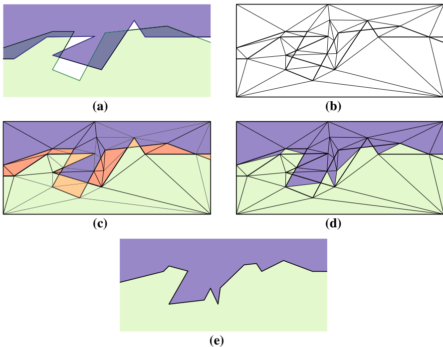
Fig. 4 a Original dataset with two polygons (same as Fig. 2). b The CT of the input polygons. c Labelling of the triangles: the colours represent the label of each polygon ( orange no label; red 2+ labels). d Triangles are relabelled such that each triangle has one and only one label. e The resulting alignment of the two polygons (colour figure online)
