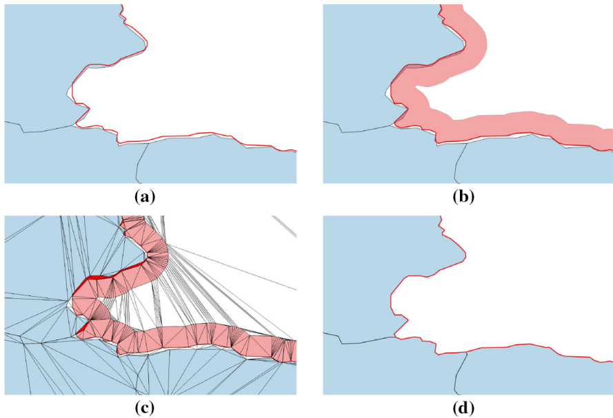
Fig. 16 a Part of the GEOFLA dataset with an international boundary ( red line ). b Creation of a polygon from the boundary ( red polygon ). c The labelled CDT. d GEOFLA correctly aligned to the boundary (colour figure online)
