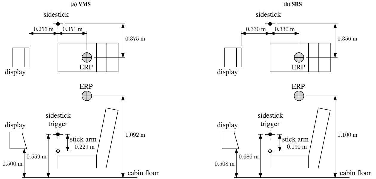
Fig. 9 Simulator cockpit dimensions.
