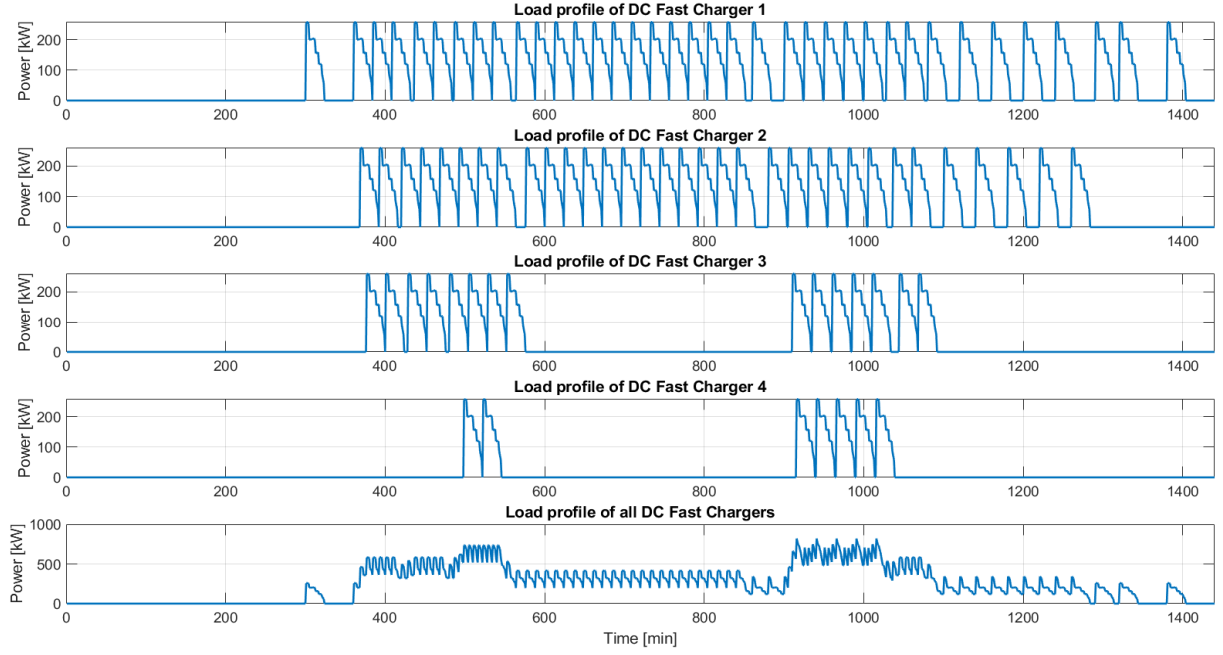
Fig. 6: The load profile of the fast-charging station
