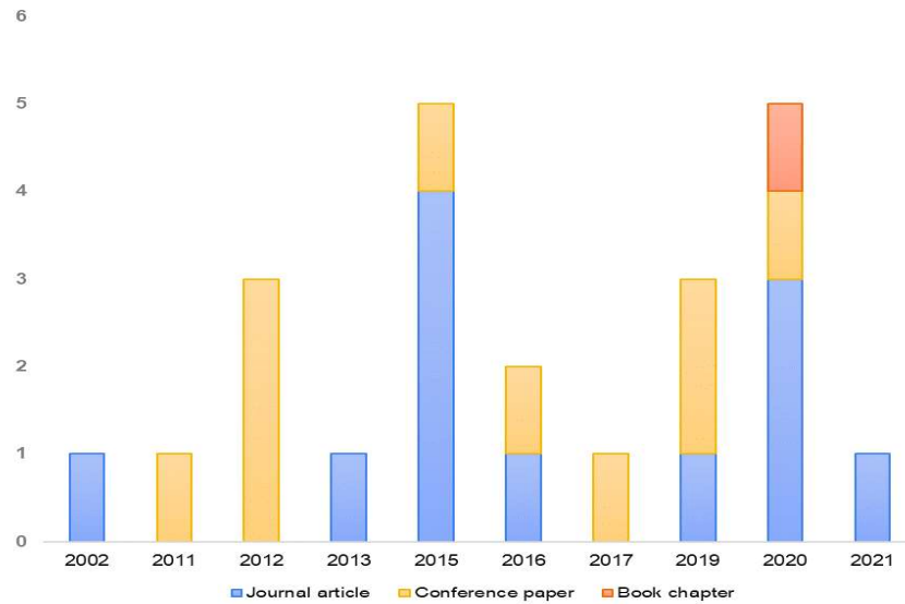
Fig. 1. Distribution of publication's number across the years
