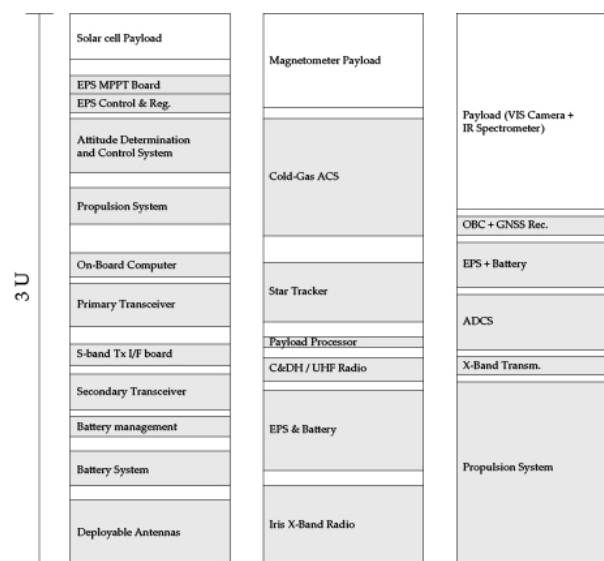
Figure 9. Volume budgets for Delfi-n3Xt, INSPIRE, and the instantiated architecture (from left to right).
