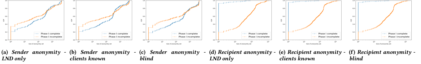
Figure 2: Distribution of the sizes of the sender and recipient anonymity set sizes.
