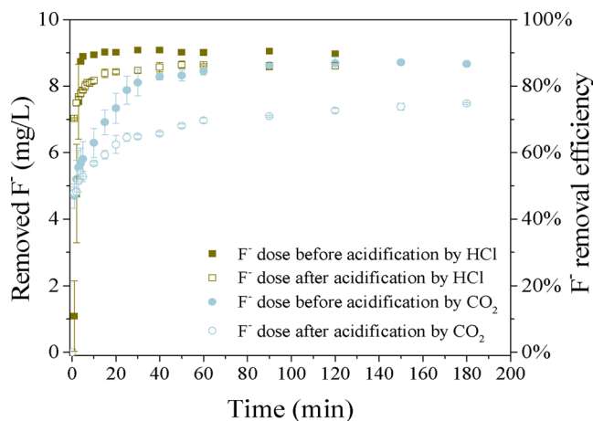
Fig. 4. F^- removal capacity and removal percentage, as a function of time. Initial F^- = 10 mg/L; pH = 6; LDHs dose = 1 g/L; T = 22 \pm 1^\circ\text{C} .
