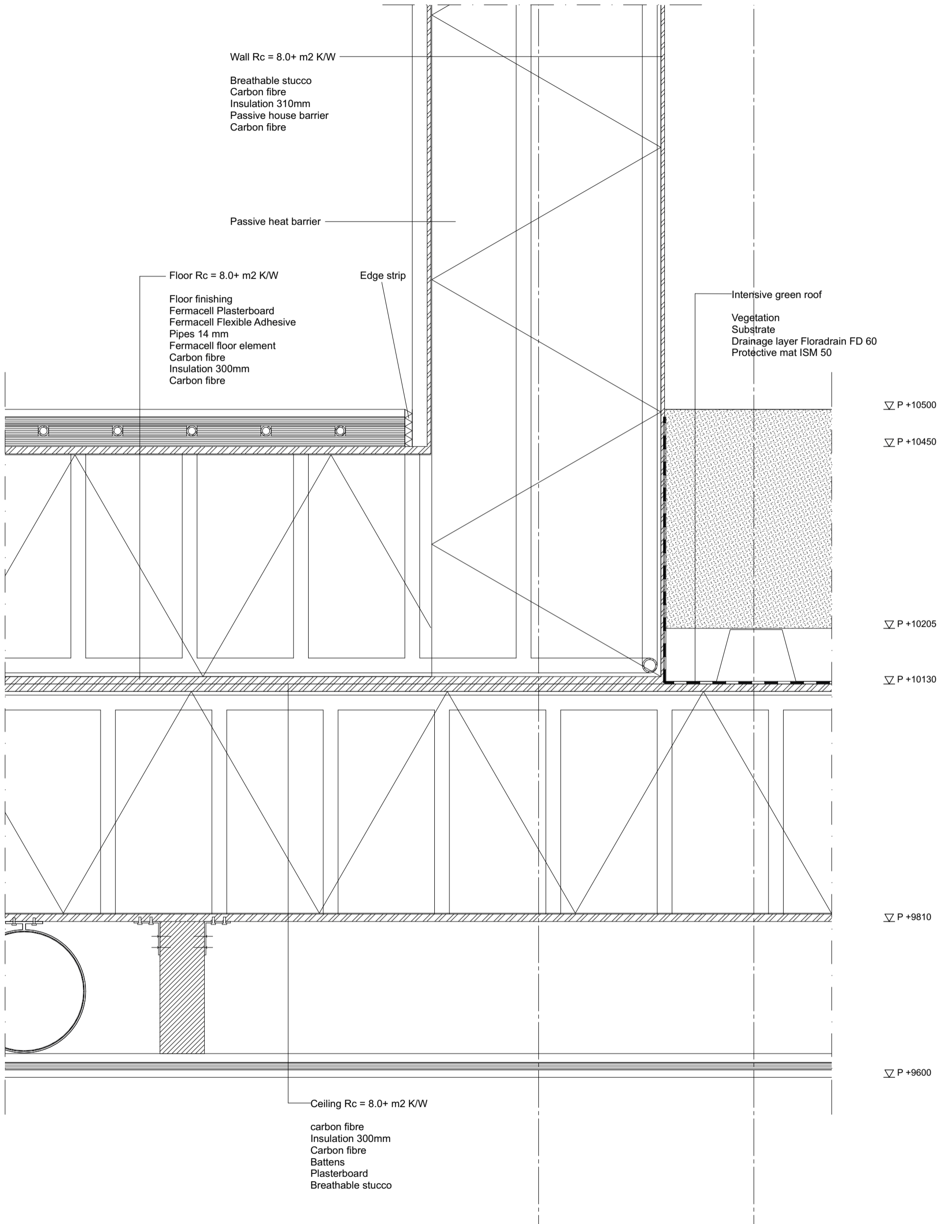
Floor - ceiling - green roof 7.17 DETAIL
