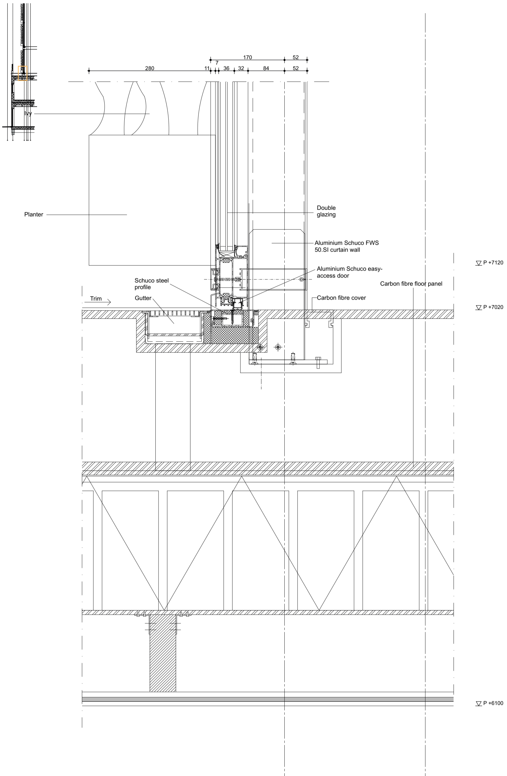
Under connection curtain wall door staircase 7.08 DETAIL
