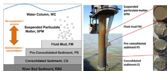
Figure 2: Schematic of sediment layers from top to bottom: suspended particulate matter (SPM), fluid mud (FM), pre-consolidated sediment (PS) consolidated sediment (CS) and riverbed sediment (RBS).
