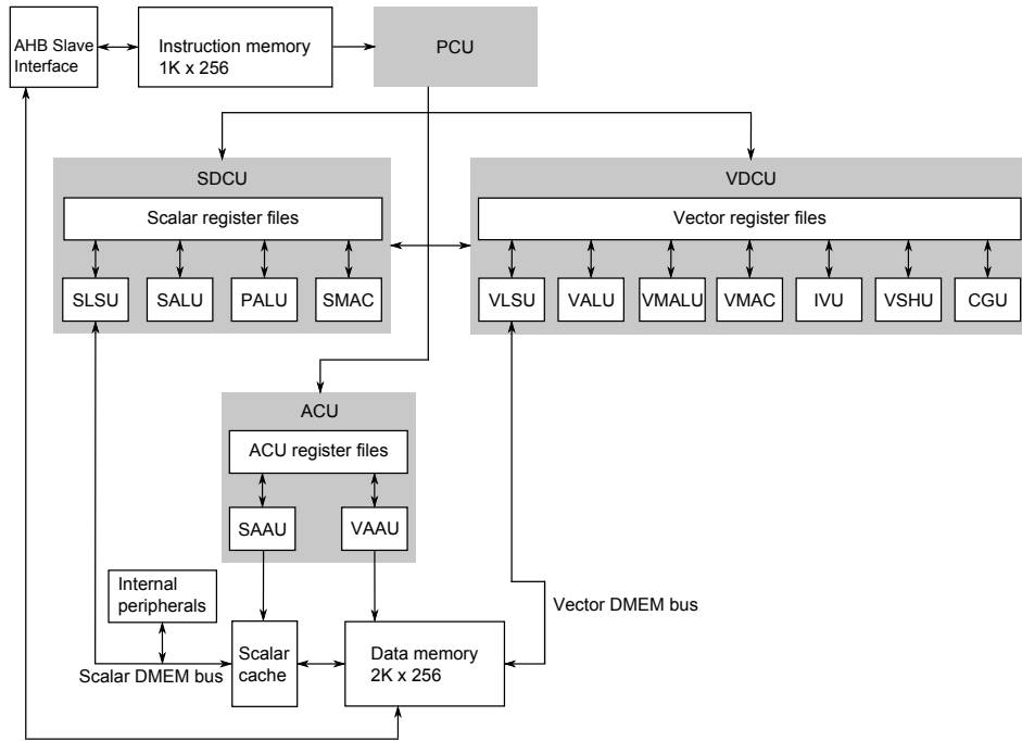
Figure 2.1: EVP functional block diagram [33]
