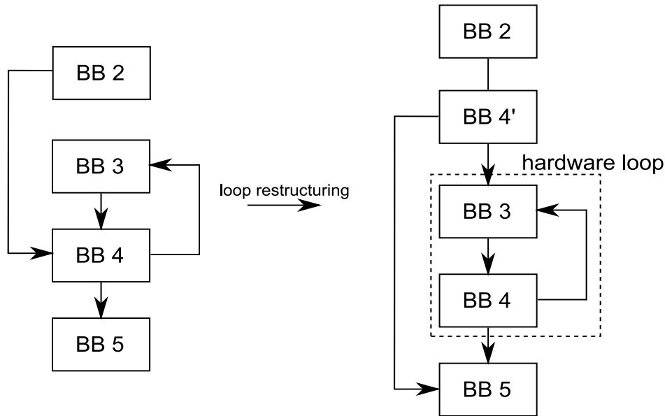
Figure 3.2: Loop restructuring to enable hardware loop generation
