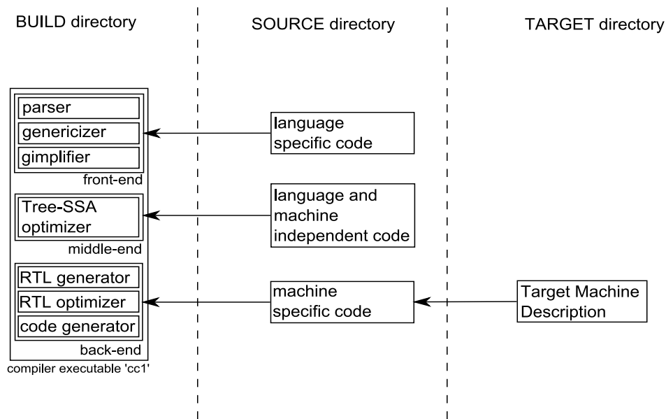
Figure 2.3: Files used in building the GCC compiler executable
