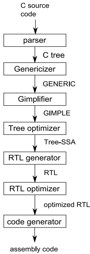
Figure 2.4: Compiler flow of the GCC compiler
