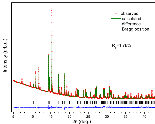
Figure 1. SR XRD powder diffraction pattern of CeMgSn collected using the multipurpose diffractometer at BM01, SNBL, ESRF, Grenoble, France, using a wavelength of 0.75334 Å. R_{\text{prof}} = 0.0176 . The vertical bars at the bottom and the blue line indicate the angles of the Bragg reflections used to simulate the refined pattern and the difference between the measured and refined patterns, respectively.
