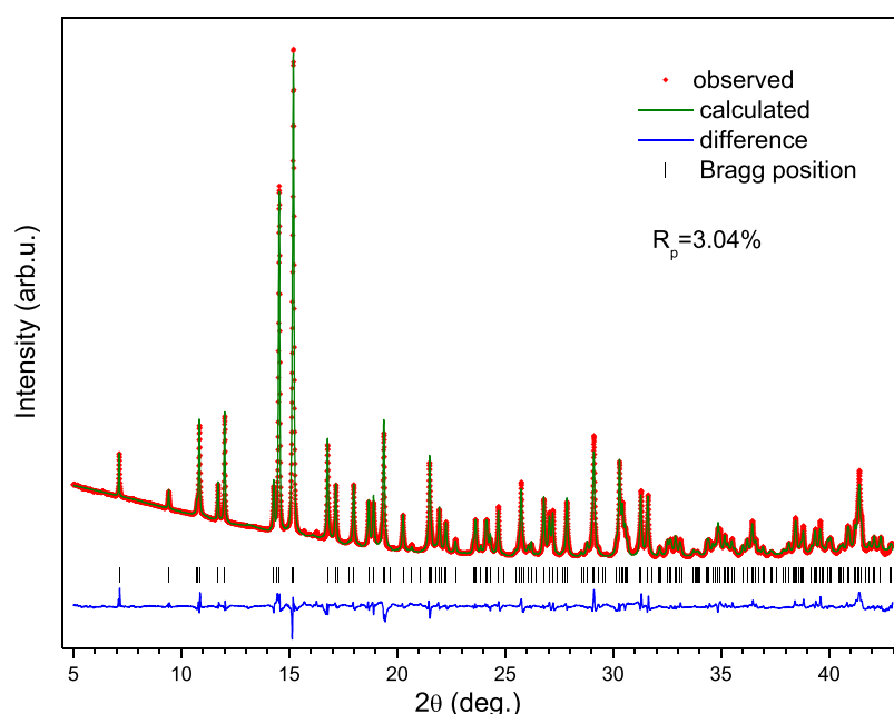
Figure 3. SR XRD pattern of CeMgSnD collected with a multipurpose diffractometer at BM01, SNBL, ESRF, Grenoble, France, using a wavelength of 0.75334 Å. R_{\text{prof}} = 0.0304 . The vertical bars in the row below the pattern indicate the positions of the Bragg reflections used to calculate the refined pattern. Shown below is the difference between the observed and refined patterns.
