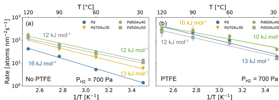
Figure 7. Arrhenius plots of the hydrogen absorption rate at P_{H_2} = 700 Pa of 40 nm Ta thin films capped with 10 nm Pd_{1-y}Au_y , (a) without and (b) with a 30 nm PTFE layer on top of the capping layer. The solid lines indicate fits to the Arrhenius equation of eq 2 and the numbers indicate the apparent activation energy obtained from the fits.
