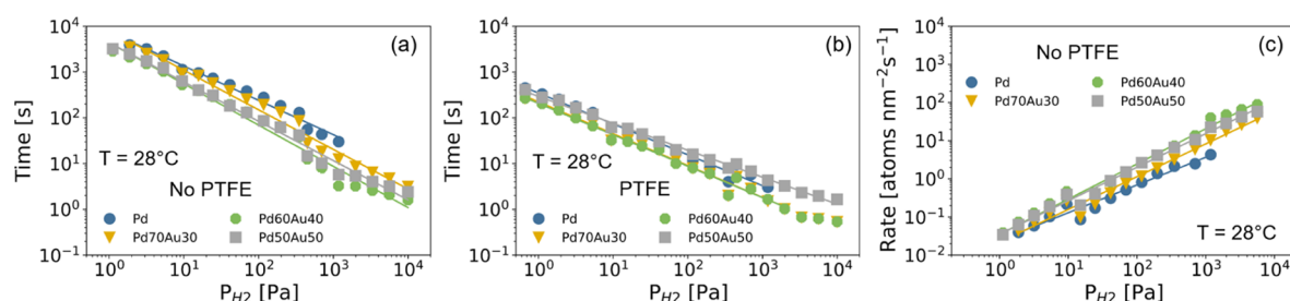
Figure 4. Hydrogen absorption kinetics of 40 nm Ta thin films capped with 10 nm Pd 1-y Au y at T = 28 °C. Hydrogen pressure dependence of the response time (a) without and (b) with a 30 nm PTFE layer on top of the capping layer. The solid lines indicate fits to a power law ( t_{\text{response}} = a \cdot P_{\text{H}_2}^\gamma ). The response time is defined as the time to reach 90% of the total signal in Figure 3. (c) Pressure dependence of the hydrogen absorption rate R computed according to eq 1. The solid lines indicate fits to a power law ( R = a \cdot P_{\text{H}_2}^\gamma ) for which the exponents \gamma are reported in Table 1.
