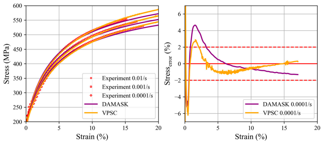
Figure 9. (Left) Experimental tensile test curves at different strain rates compared to simulated curves resulting during the calibration process using VPSC with GSODF full texture and Crystal Plasticity Finite Element Method (CPFEM) with RVE_{ODF20} . (Right) Strain dependence of the error of the predicted stress relative for the 0.0001/s tensile curve (first, cubic spline interpolation was applied for 0 to 0.2 strain and 500 points).
