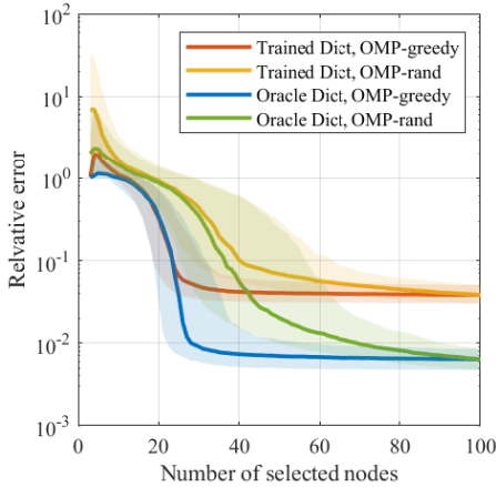
Figure 2. Performance comparison for using trained and exact dictionary. Solid lines and shaded areas indicate the medium and inter-quartile ranges.
