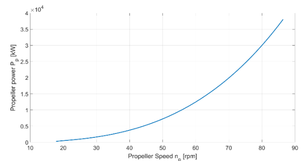
Figure 7. Required propeller power as function of rotational speed.
