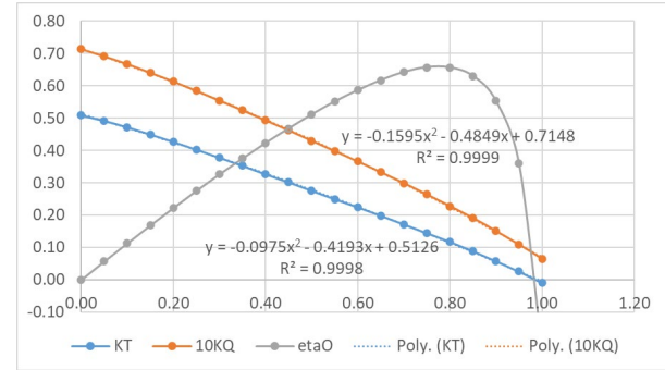
Figure 5. Open water diagram based on data in [10] with 2 nd degree polynomial fit equations.
