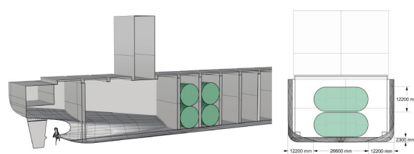
Figure 20. Integration of four 3000 m 3 ammonia tanks at the expense of 514 TEU container carrying capacity.
