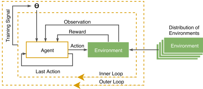
Fig. 7. Schematic of meta-RL [123].
