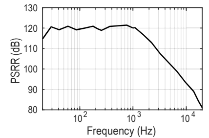
Fig. 6. Measured PSRR.
