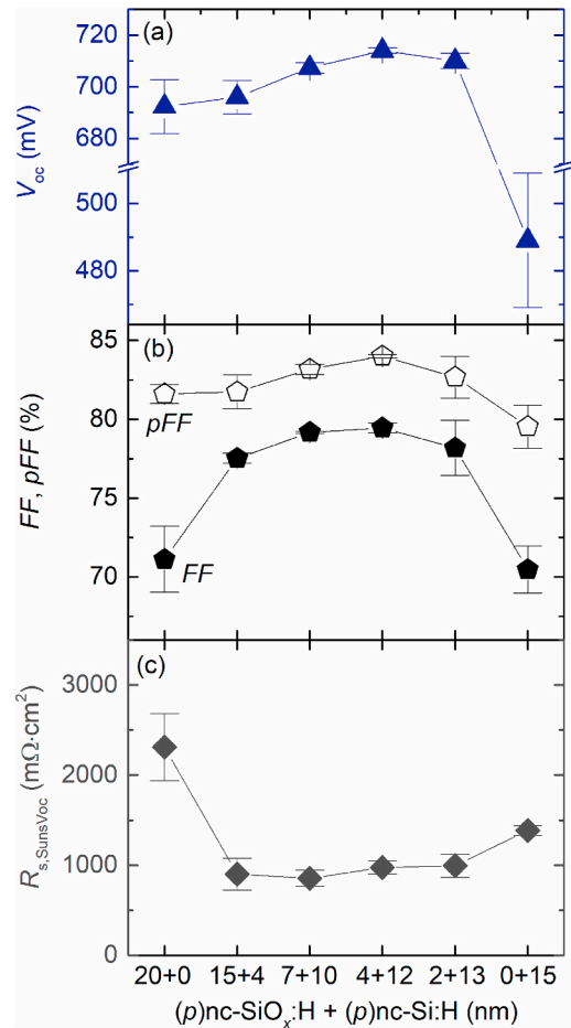
Fig. 9. Front junction FBC-SHJ solar cells with varying thicknesses of (p)-contact (p)nc-SiO x :H + (p)nc-Si:H: (a) V_{oc} ; (b) FF and pFF ; (c) R_{s,SunsVoc} . Solar cells feature a nominal 4.4% front metal coverage. The results represent averaged parameters from three solar cells. The error bars represent the standard deviations.
