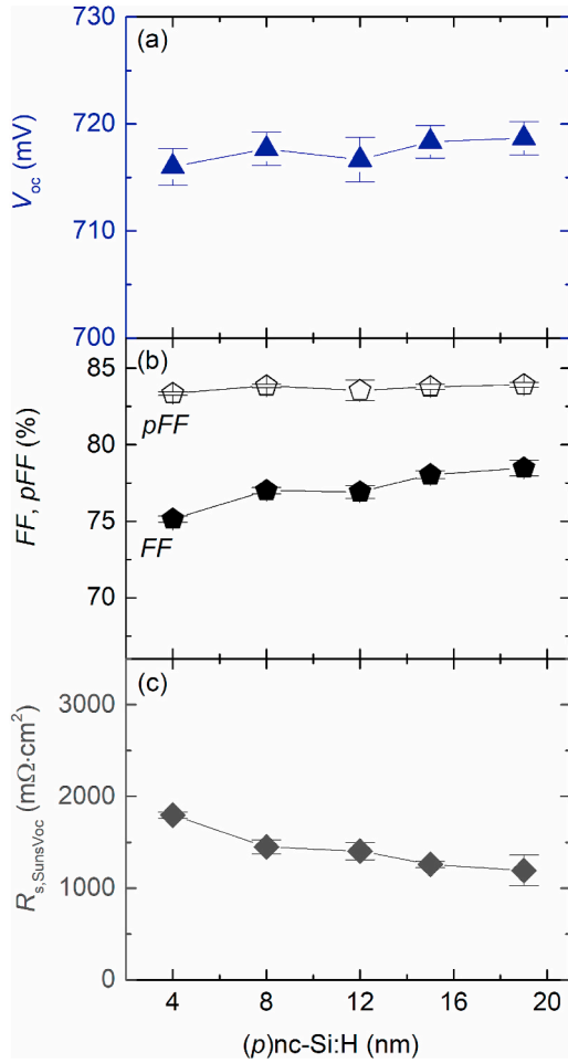
Fig. 10. Rear junction FBC-SHJ solar cells with (p) -contacts featuring a fixed 4-nm thick (p)nc-SiO_x:H but varying (p)nc-Si:H layer thicknesses: (a) V_{oc} ; (b) FF and pFF ; (c) R_{s,SunsVoc} . Solar cells feature a nominal 4.4% metal coverage. The results represent averaged parameters from three solar cells. The error bars represent the standard deviations.
