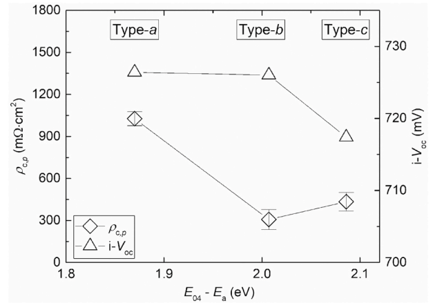
Fig. 5. The contact resistivity \rho_{c,p} and i\text{-}V_{oc} of (p)-contact stacks with (p)nc-SiO x :H layers featuring various E_{04} - E_a . The passivation quality of the symmetrical test samples was measured before ITO sputtering. The results present averaged \rho_{c,p} from two symmetrical samples and the error bars represent the standard deviations.
