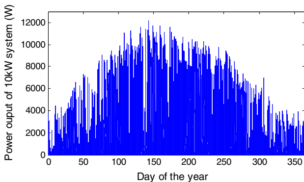
Fig. 5. Power output of 10 kW PV system as a function of time for 2013. The PV modules were oriented south with a tilt angle of 28°.
