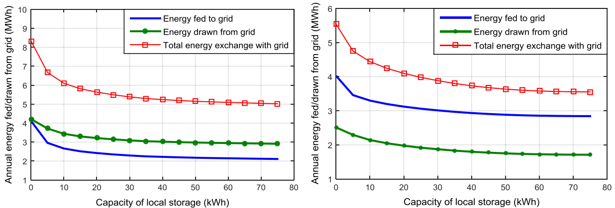
Fig. 16. Annual Energy exchanged with the grid for 2013 as a function of storage size, considering EV loads for 7 days/week (left) and only on weekdays (right) using Gaussian EV profile G4.
