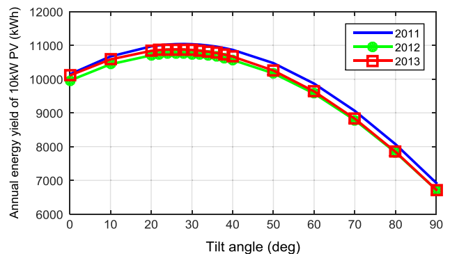
Fig. 4. Annual energy yield of 10 kW PV system as a function module tilt for years 2011–13. The PV modules were oriented south with azimuth of 0°.
