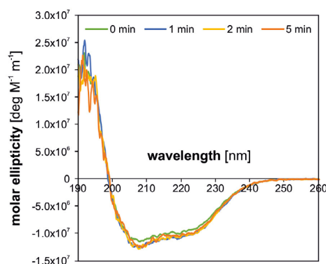
Figure 4. CD spectra of HRP after exposure to plasma. HRP (110 \mu\text{L} ) was treated as described above for activity measurements and diluted 1:5, which corresponds to 0.2 \text{mg mL}^{-1} for the untreated sample. Immediately after treatment, the sample was transferred to a suitable cuvette and subjected to CD measurements. CD spectra were normalized with respect to protein concentration as determined by the Bradford method.
