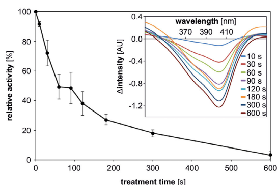
Figure 3. HRP inactivation by plasma treatment. Plasma treatment was performed with 110 \mu\text{L} HRP (1 \text{kU mL}^{-1} ) in KPi buffer (100 mM, pH 6.5) without guaiacol. Activity was measured by diluting the treated samples to 0.1 \text{U mL}^{-1} in KPi buffer including 5 mM of guaiacol and subsequent addition of \text{H}_2\text{O}_2 at a final concentration of 0.25 mM. Guaiacol conversion was immediately monitored at \lambda = 470 nm and activity calculated from the initial slope during the first 30 s. From the same treated samples, absorption spectra were measured with a 1:5 dilution in KPi. The inset shows the Soret band of HRP with A_{\text{max}} at \approx 403 nm. Spectra are displayed with the untreated sample as blank, thereby showing a decrease in absorbance at the Soret peak. Data were recorded in triplicate for both activity measurements and spectra.
