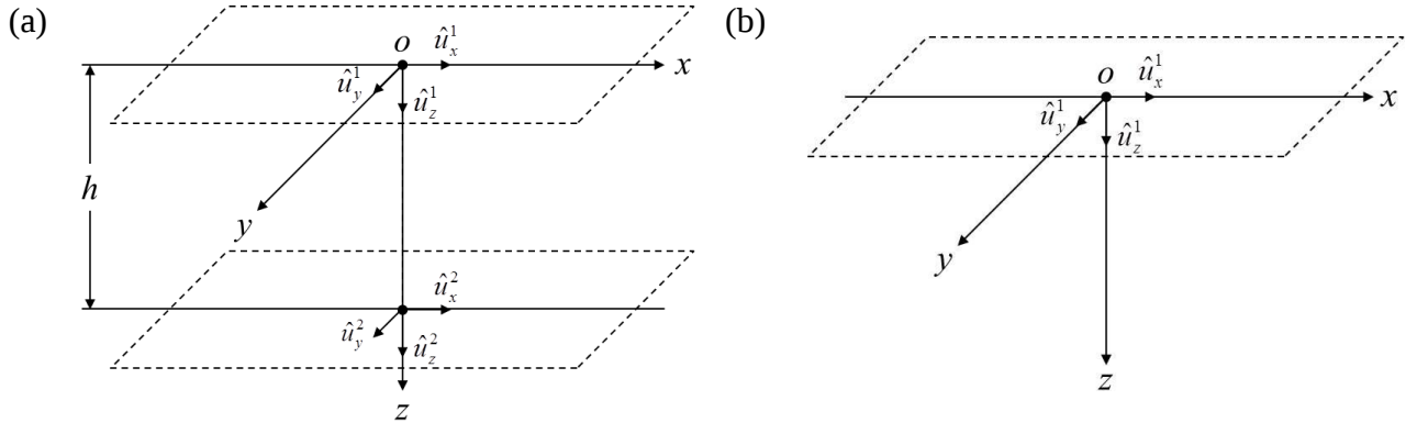
Figure 3. Schematic representation of spectral elements: (a) Layer spectral element and (b) Semi-infinite spectral element.
