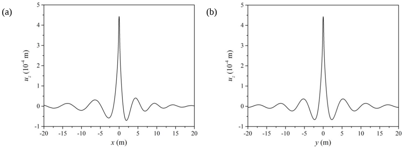
Figure 7. Profiles of u_z for points along different axes on the pavement surface for t = 0 : (a) x -axis and (b) y -axis.
