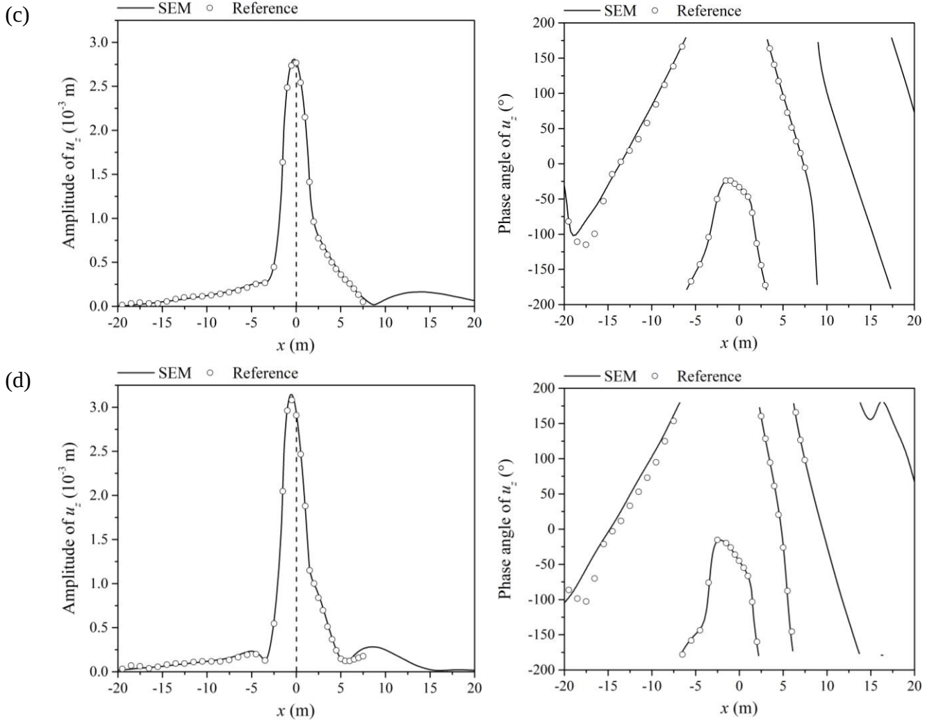
Figure 5. Comparison of u_z for points along the x -axis on the layered system surface calculated by different methods at different moving velocities: (a) c = 0 m/s, (b) c = 25 m/s, (c) c = 50 m/s, and (d) c = 75 m/s.
