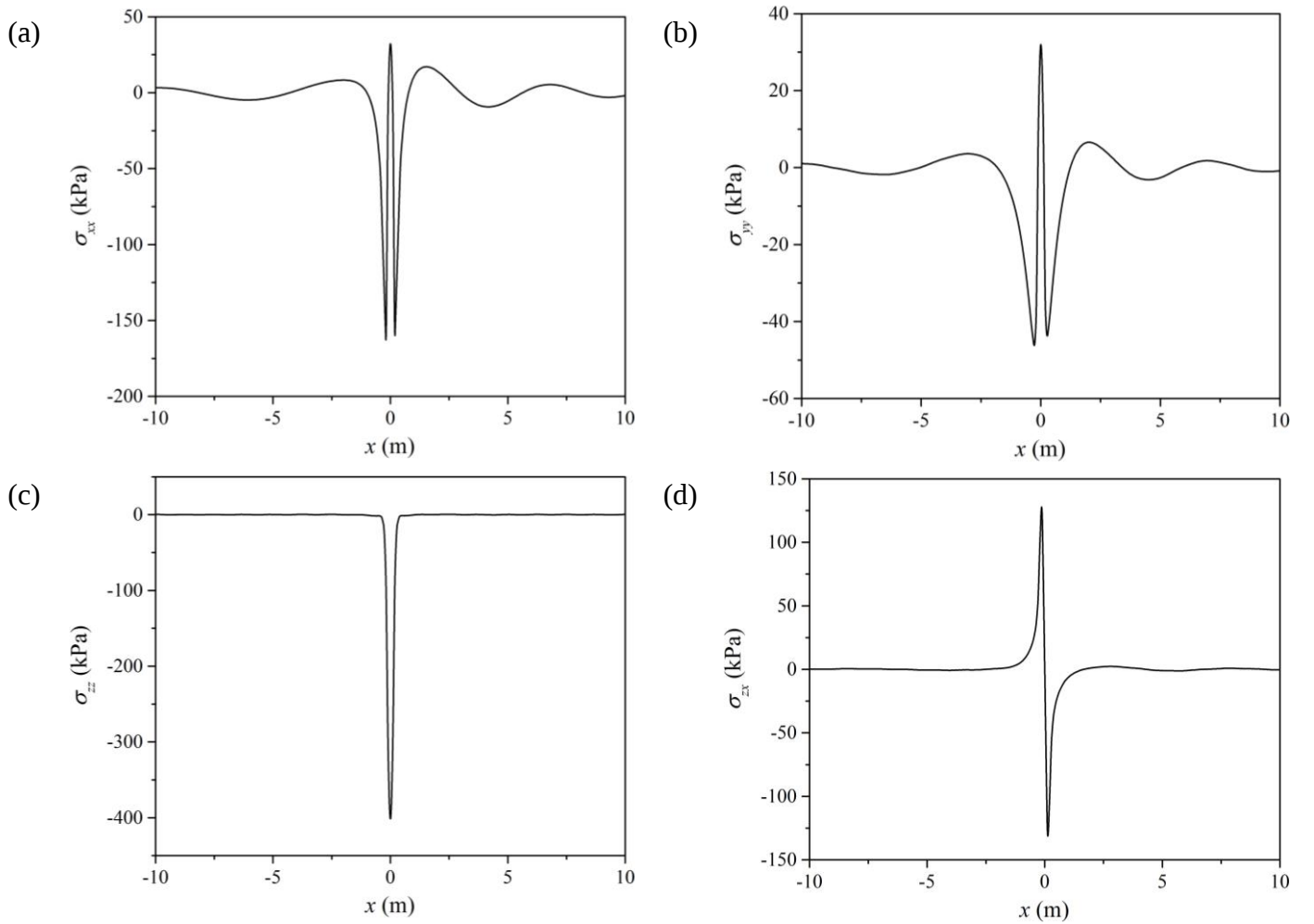
Figure 8. Stresses of points along the x -axis at depth 0.1 m for t = 0 :
