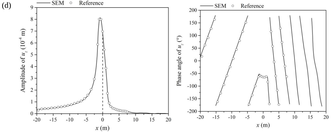
Figure 4. Comparison of u_z for points along the x -axis on the half-space surface calculated by different methods at different moving velocities:
